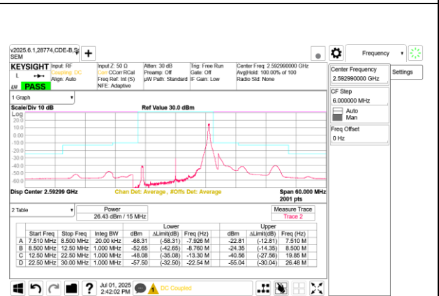
5G NR n41 15MHz BPSK Mid Channel RB1-37 Port B
