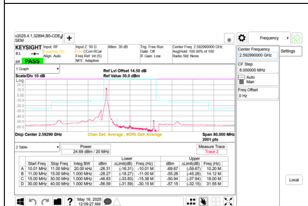
5G NR n41 20MHz BPSK Middle Channel RB1-0 Port B
