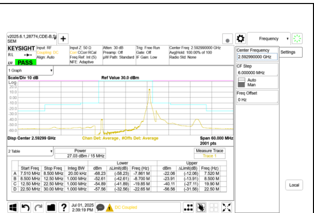
5G NR n41 15MHz BPSK Mid Channel RB1-37 Port A
