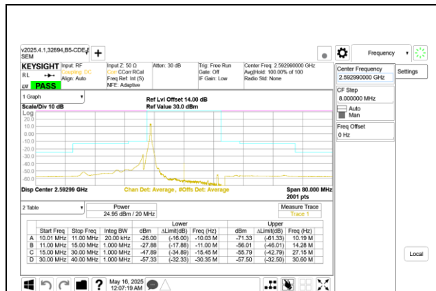
5G NR n41 20MHz BPSK Middle Channel RB1-0 Port A
