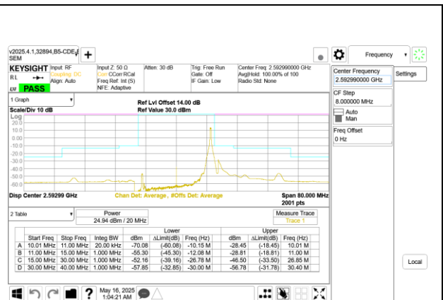
5G NR n41 20MHz BPSK Mid Channel RB1-50 Port A
