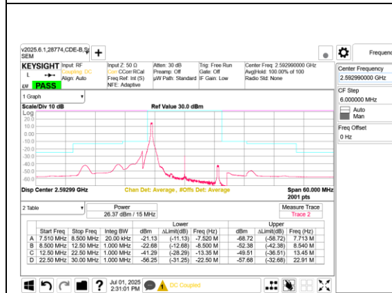
5G NR n41 15MHz BPSK Middle Channel RB1-0 Port B
