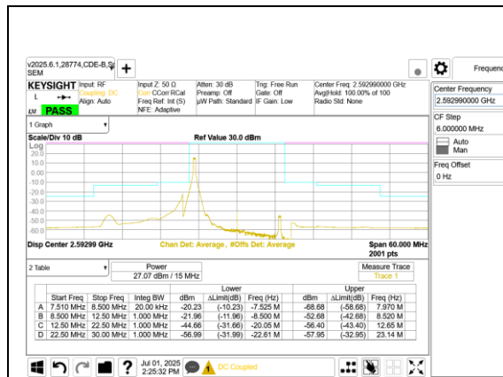
5G NR n41 15MHz BPSK Middle Channel RB1-0 Port A
