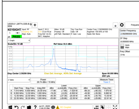
5G NR n41 15MHz BPSK Middle Channel RB1-0 Port A+B
