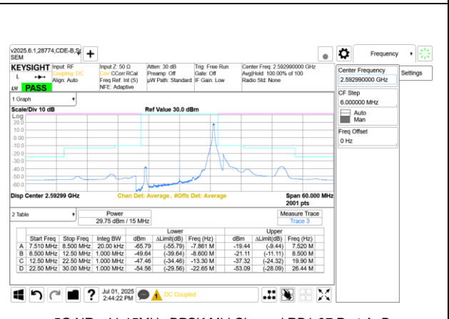
5G NR n41 15MHz BPSK Mid Channel RB1-37 Port A+B
