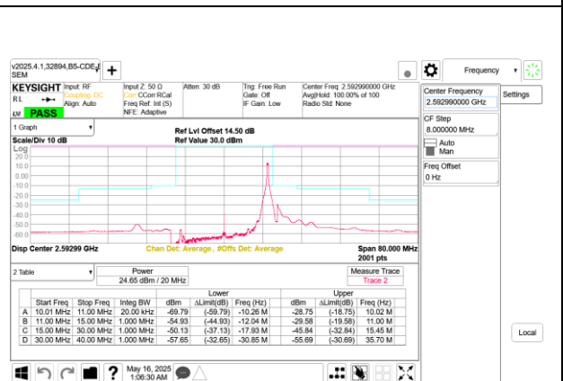
5G NR n41 20MHz BPSK Mid Channel RB1-50 Port B
