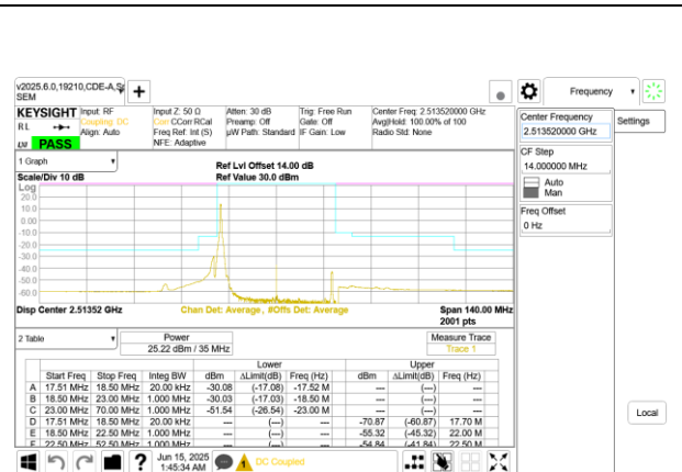
5G NR n41 35MHz BPSK Low Channel RB1-0
