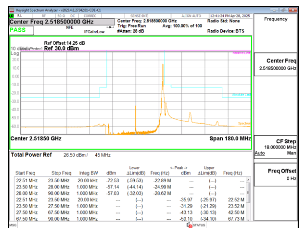
5G NR n41 45MHz BPSK Low Channel RB1-118
