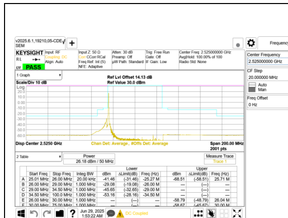
5G NR n7 50MHz BPSK Low Channel RB1-0
