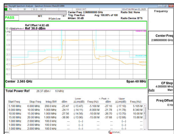
5G NR n7 10MHz BPSK High Channel RB50-0
