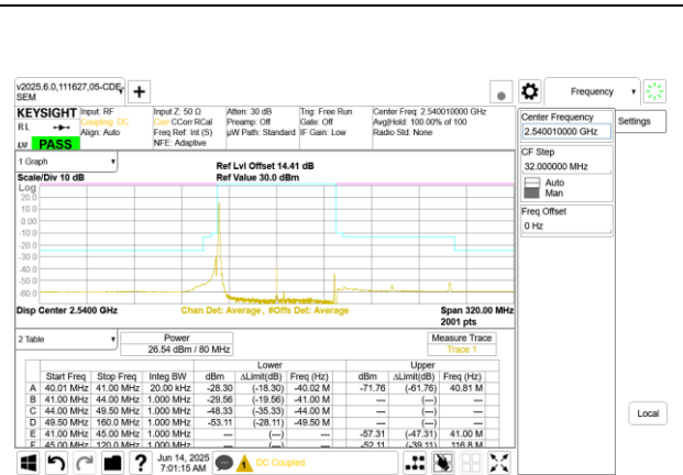
5G NR n41 80MHz BPSK Low Channel RB1-0
