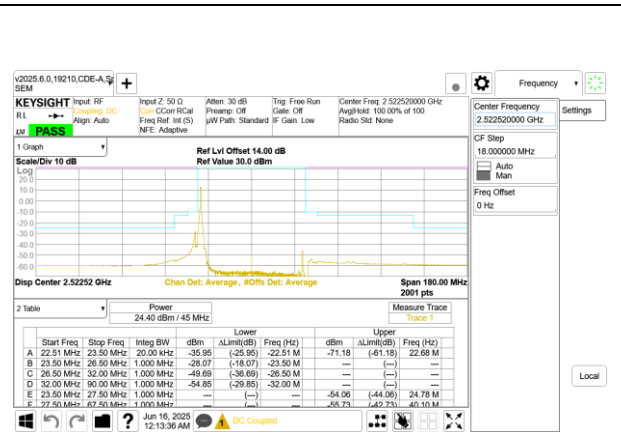
5G NR n41 45MHz BPSK Low Channel RB1-0
