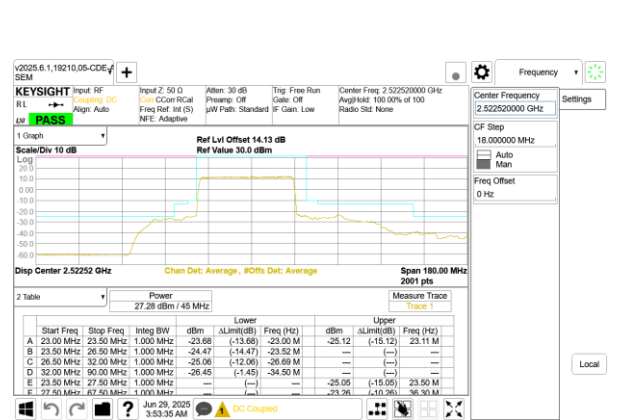
5G NR n41 45MHz BPSK Low Channel RB108-0
