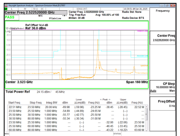
5G NR n41 45MHz BPSK Low Channel RB1-118
