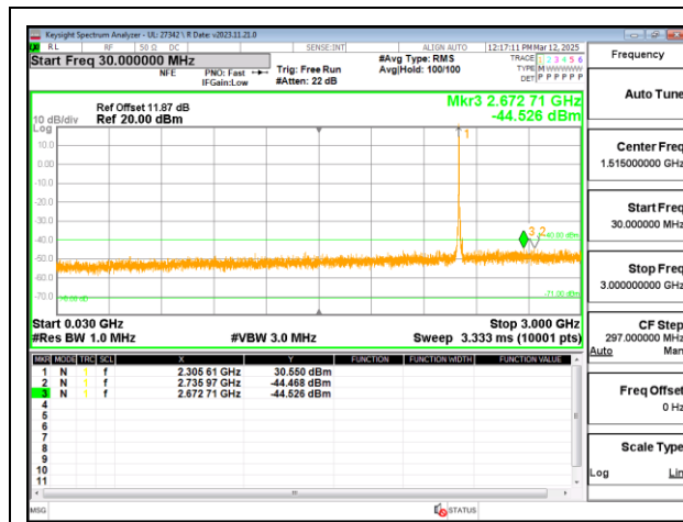
5G NR n30 10MHz BPSK Middle Channel RB1-1 (30MHz to 3GHz)
