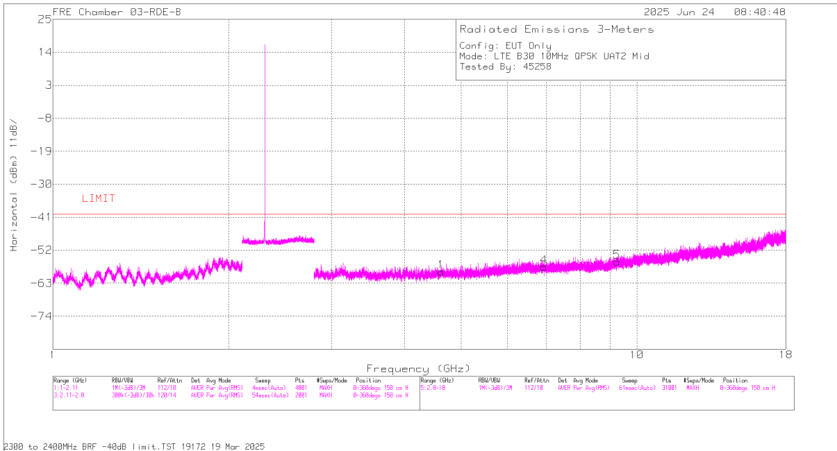
Horizontal Polarity
