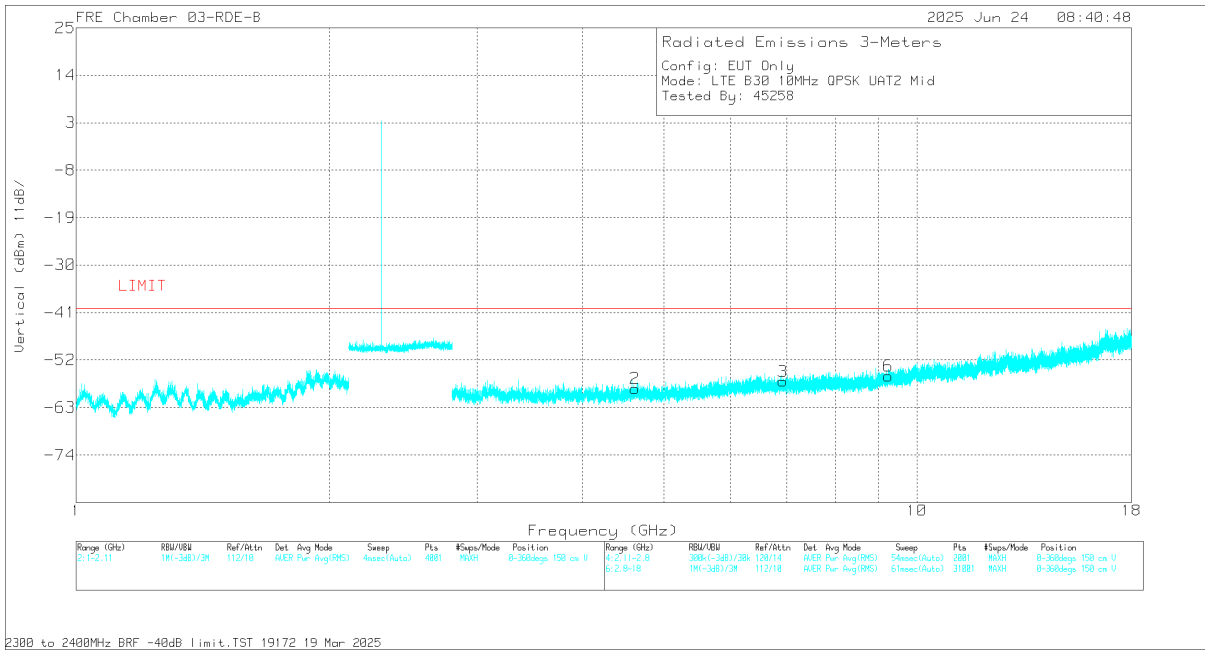
Vertical Polarity
