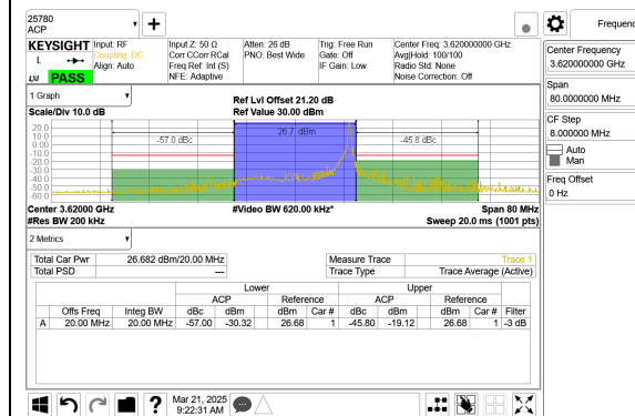
LTE B48 20MHz QPSK Middle Channel RB1-99
