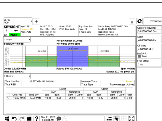
LTE B48 10MHz QPSK Middle Channel RB50-0
