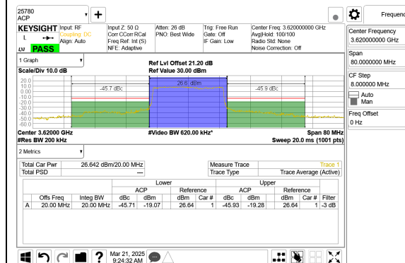
LTE B48 20MHz QPSK Middle Channel RB100-0
