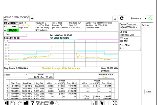
LTE B48 20MHz QPSK Low Channel RB100-0
