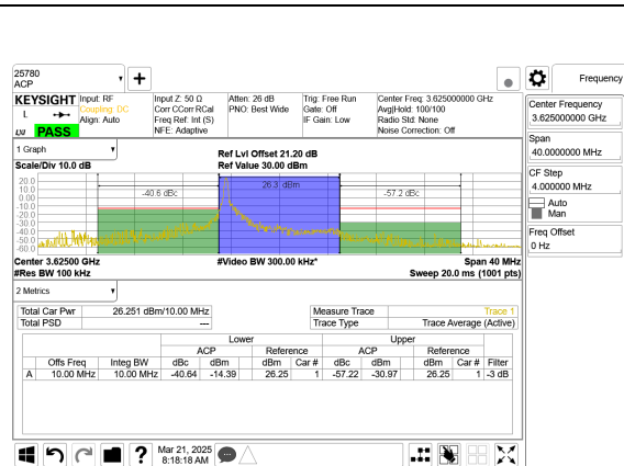
LTE B48 10MHz QPSK Middle Channel RB1-0
