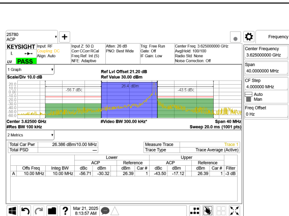
LTE B48 10MHz QPSK Middle Channel RB1-49
