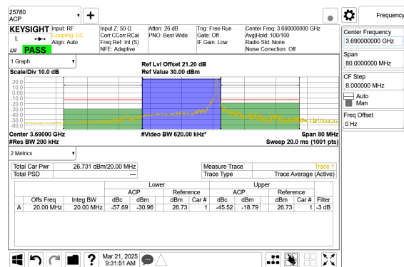
LTE B48 20MHz QPSK High Channel RB1-99
