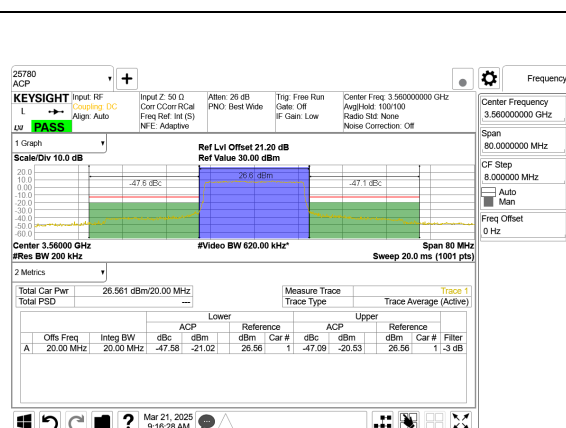
LTE B48 20MHz QPSK Low Channel RB100-0
