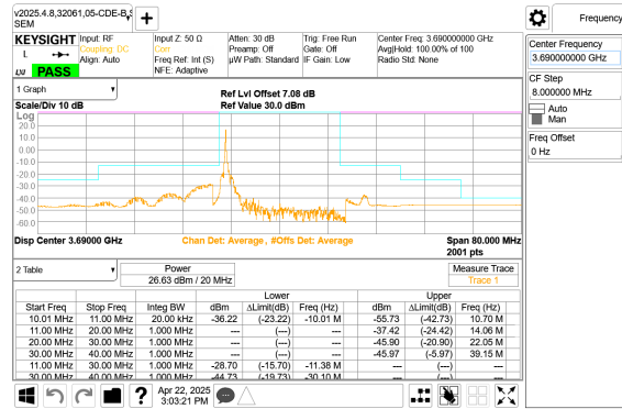
LTE B48 20MHz QPSK High Channel RB1-0
