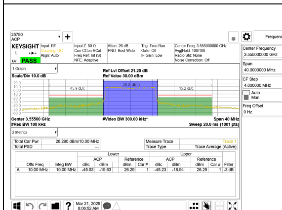
LTE B48 10MHz QPSK Low Channel RB50-0
