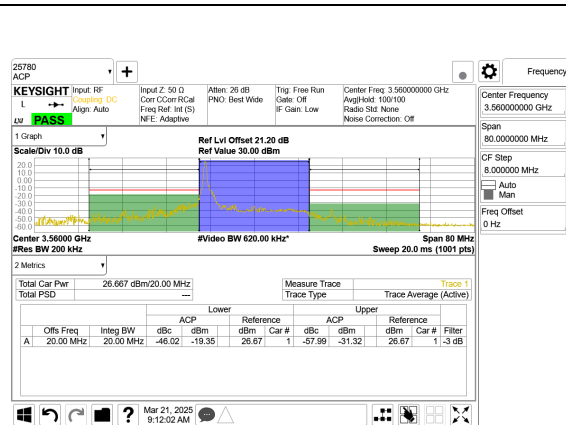
LTE B48 20MHz QPSK Low Channel RB1-0
