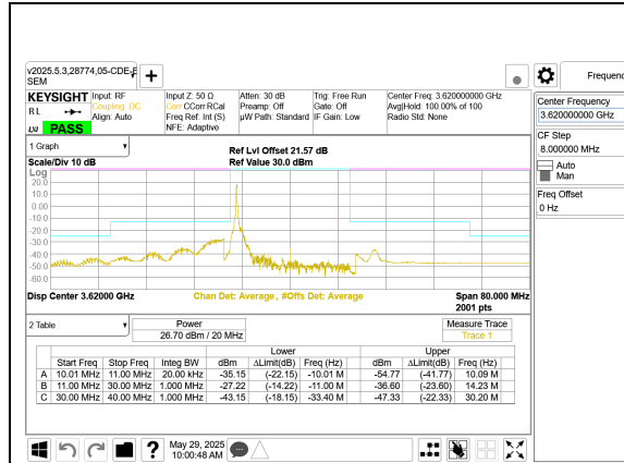
LTE B48 20MHz QPSK Middle Channel RB1-0
