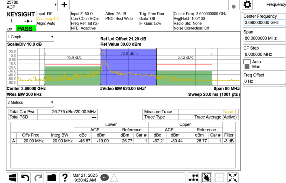
LTE B48 20MHz QPSK High Channel RB1-0
