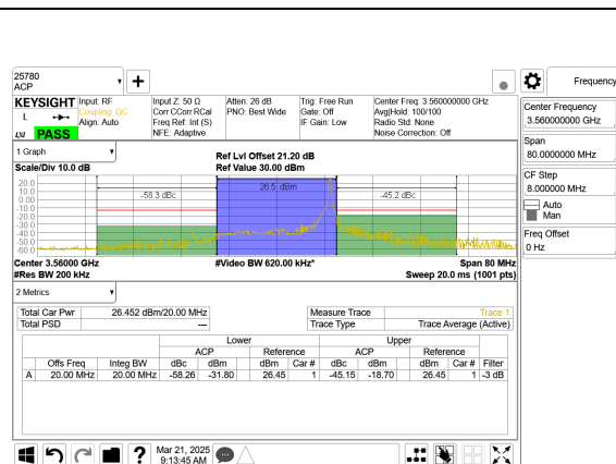
LTE B48 20MHz QPSK Low Channel RB1-99
