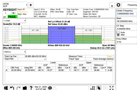
LTE B48 20MHz QPSK High Channel RB100-0
