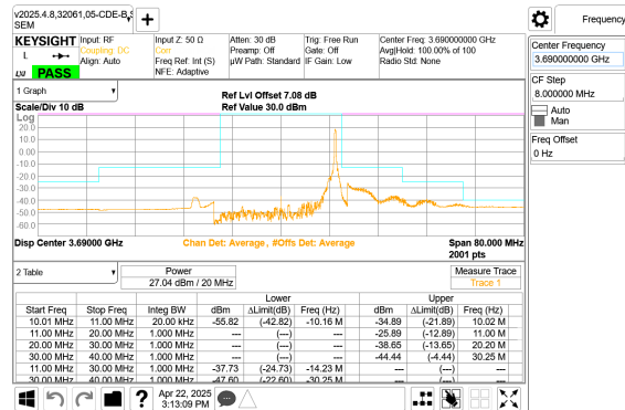
LTE B48 20MHz QPSK High Channel RB1-99
