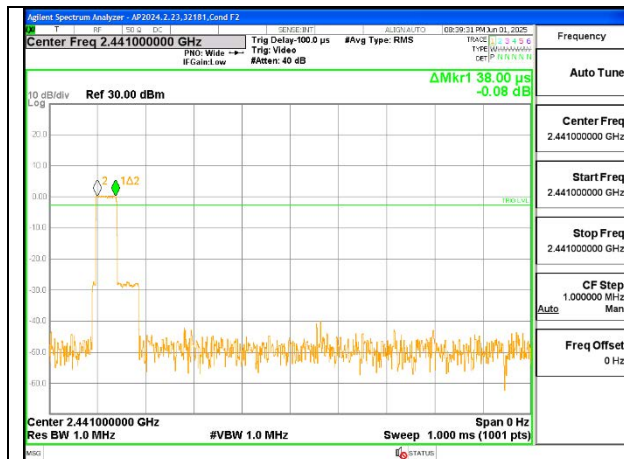
PULSE WIDTH – 2Mbps
