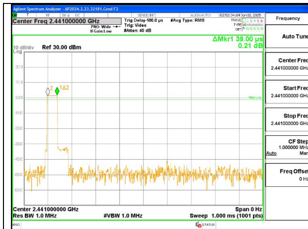
PULSE WIDTH – 2Mbps
