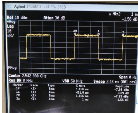
Figure 4: 5G NR TDD Power Class 2, 50% RB
