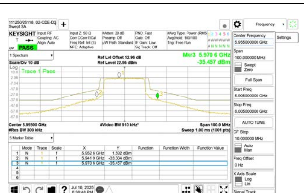
LOW CHANNEL ANT 5 5955
