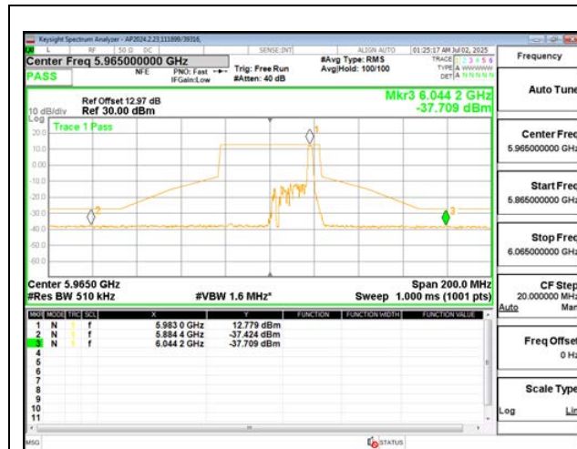
LOW CHANNEL ANT 5 5965
