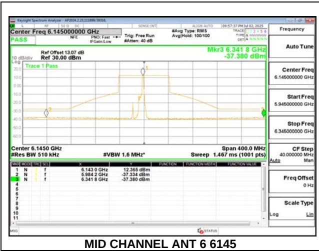
MID CHANNEL ANT 6 6145
