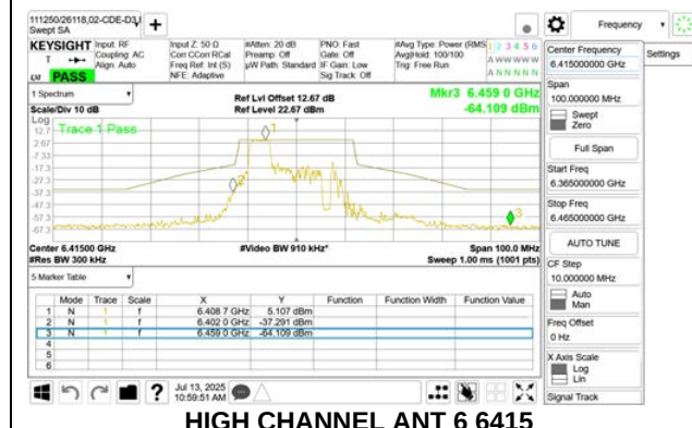
HIGH CHANNEL ANT 6 6415
