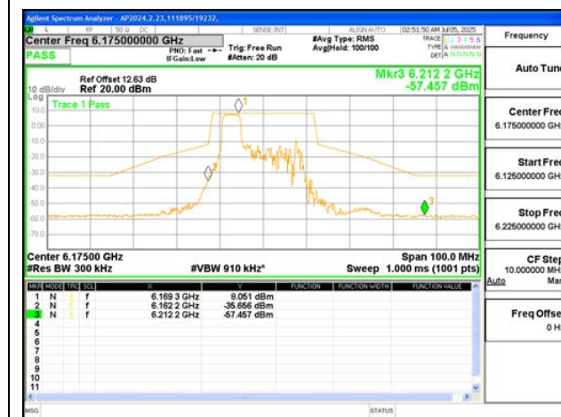
MID CHANNEL ANT 6 6175
