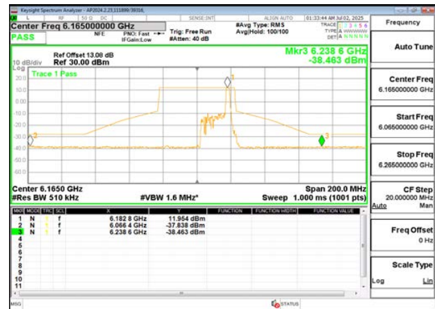
MID CHANNEL ANT 5 6165
