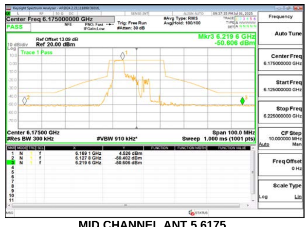
MID CHANNEL ANT 5 6175
