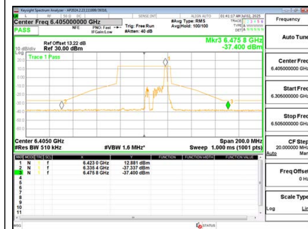
HIGH CHANNEL ANT 5 6405
