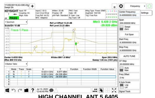
HIGH CHANNEL ANT 5 6405
