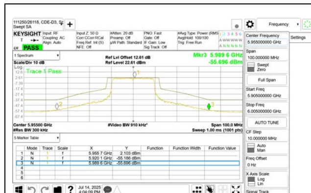
LOW CHANNEL ANT 6 5955
