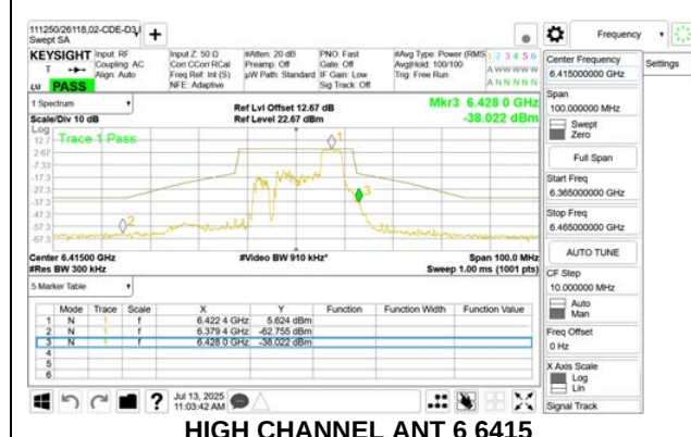
HIGH CHANNEL ANT 6 6415
