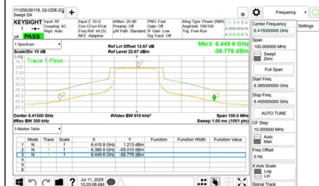
HIGH CHANNEL ANT 6 6415
