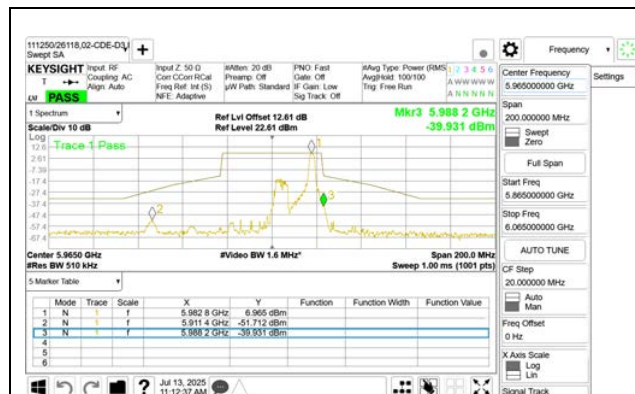
LOW CHANNEL ANT 6 5965
