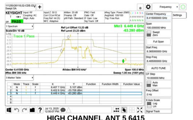
HIGH CHANNEL ANT 5 6415
