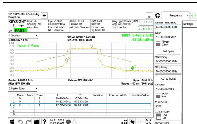
LOW CHANNEL ANT 5 6435
