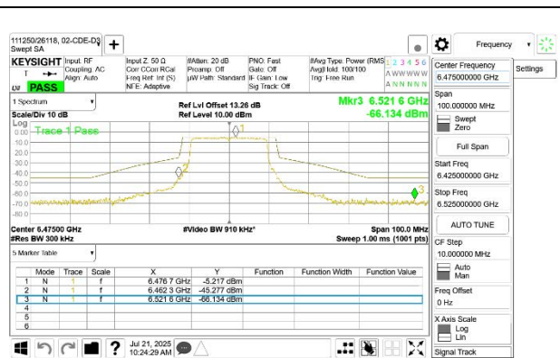
MID CHANNEL ANT 5 6475
