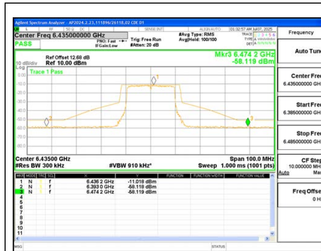
LOW CHANNEL ANT 6 6435
