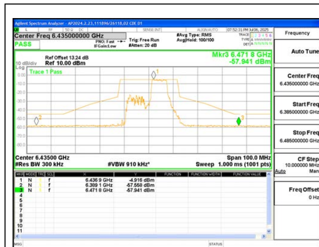
LOW CHANNEL ANT 5 6435
