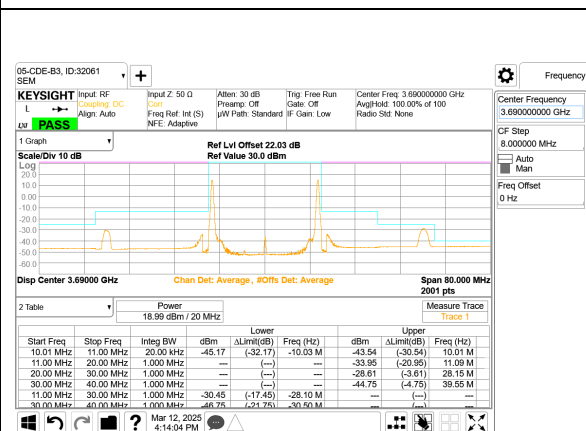
LTE ULCA B48B 10MHz + 10MHz 16QAM High Ch RB1-0 + RB1-49
