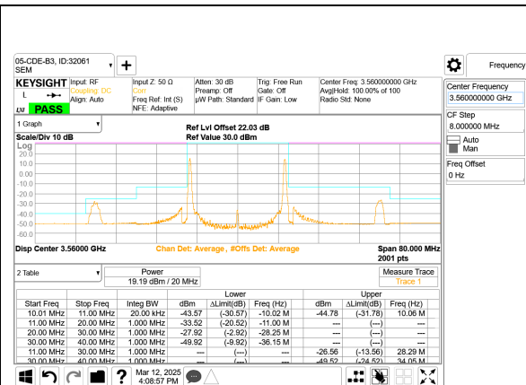
LTE ULCA B48B 10MHz + 10MHz 16QAM Low Ch RB1-0 + RB1-49
