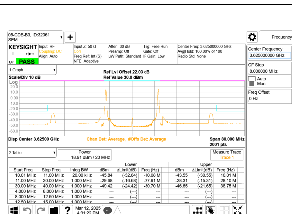
LTE ULCA B48B 10MHz + 10MHz 16QAM Mid Ch RB1-0 + RB1-49
