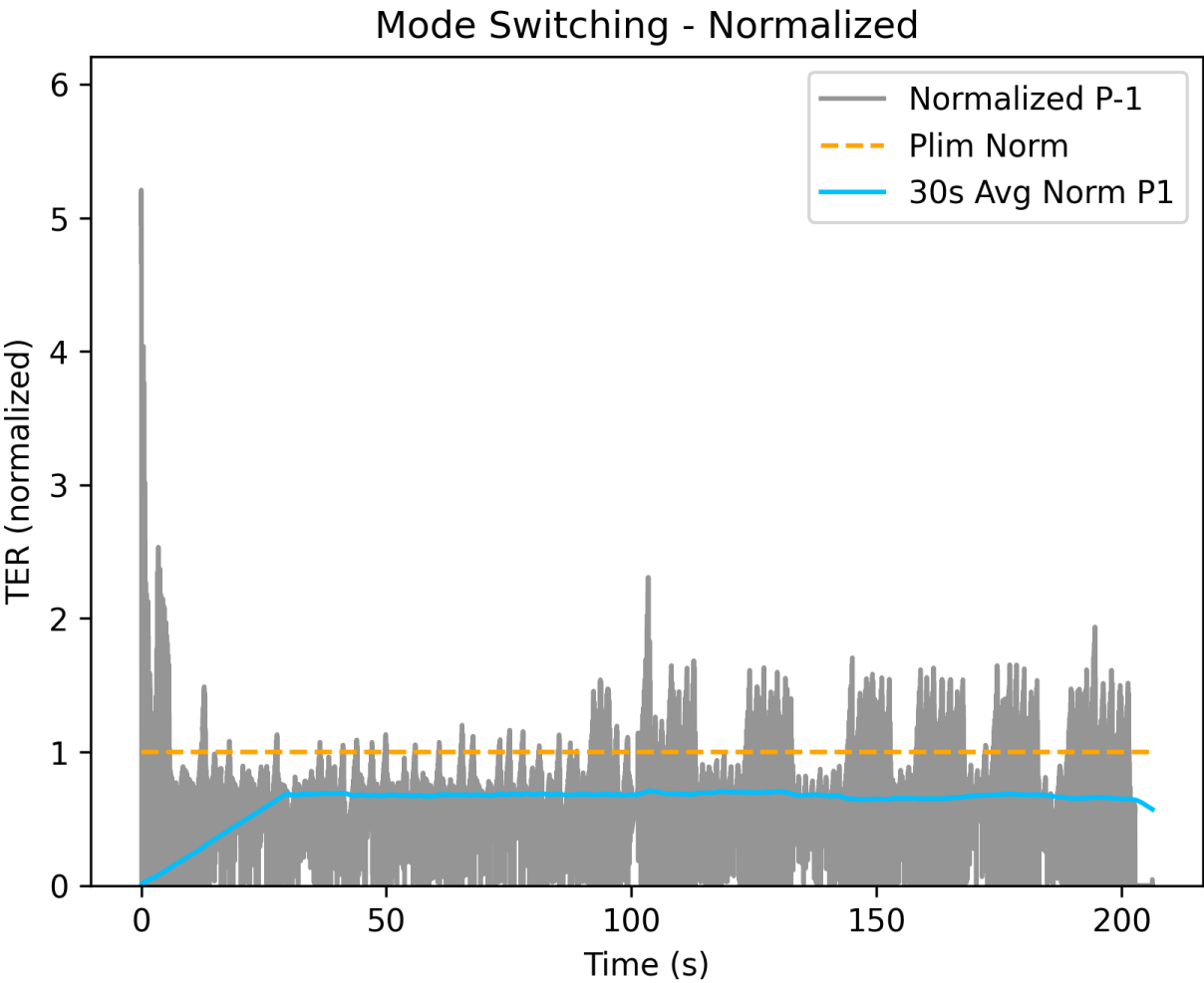
Figure 4-9: Wi-Fi Power State 3 to Power State 1 Validation
