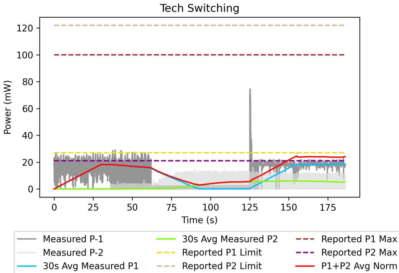
Figure 4-6: Change in Technology and Band Plot
