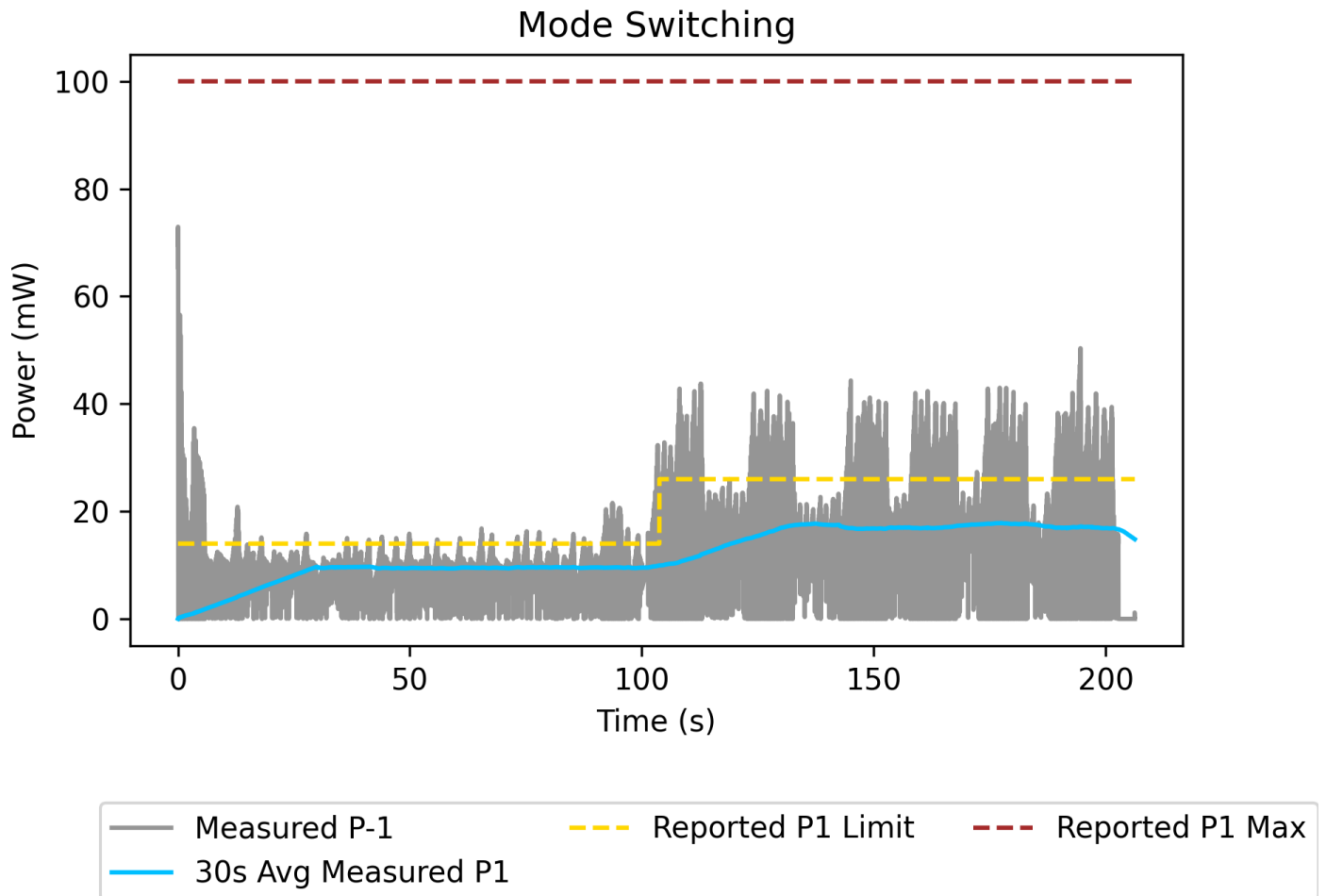
Figure 4-8: Power State 3 to Power State 1 Sequence
