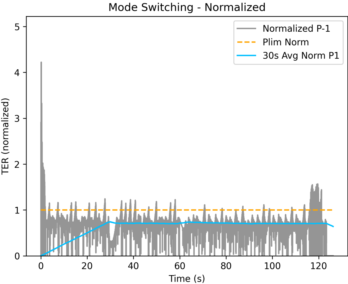
Figure 4-11: Wi-Fi Power State 3 to Power State 4 Validation
