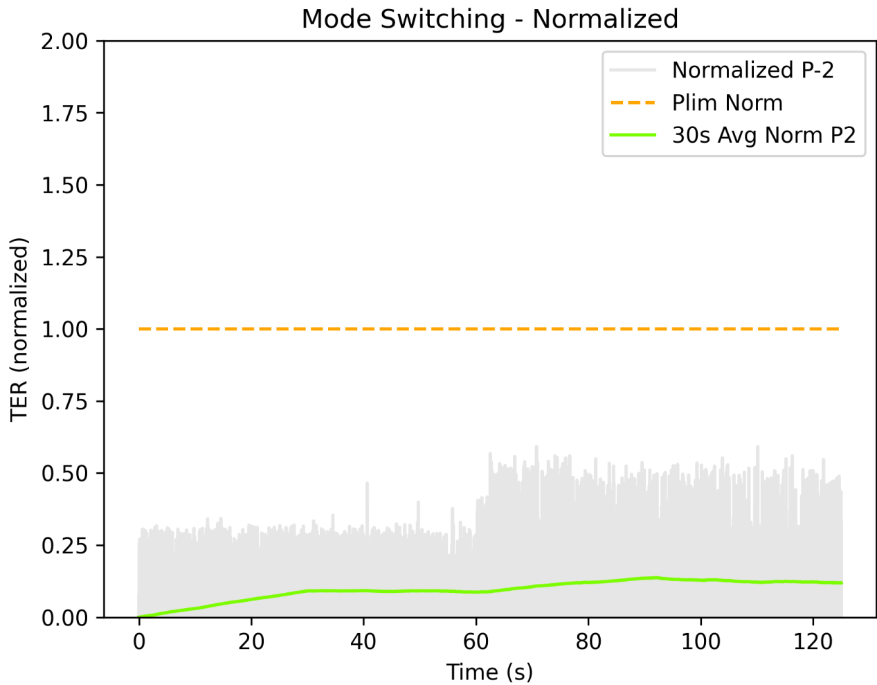
Figure 4-13: BT Power State 5 to Power State 6 Validation
