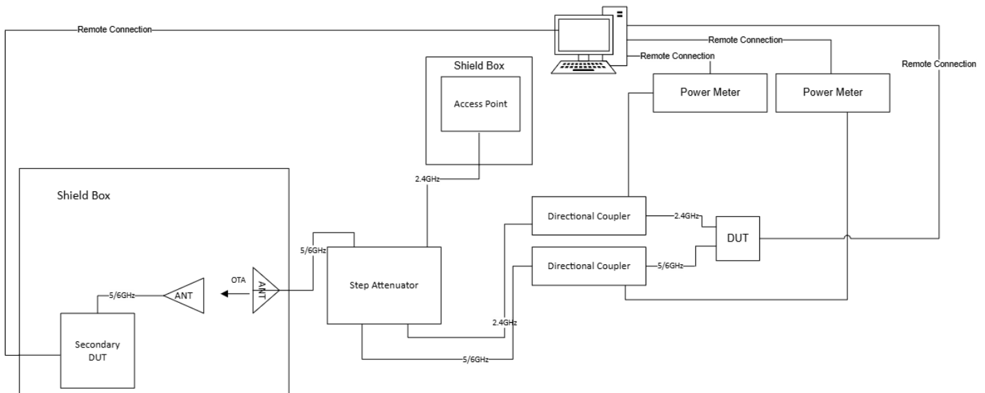
Figure 4-4: 2.4GHz to 2.4 GHz + 6GHz Switch
