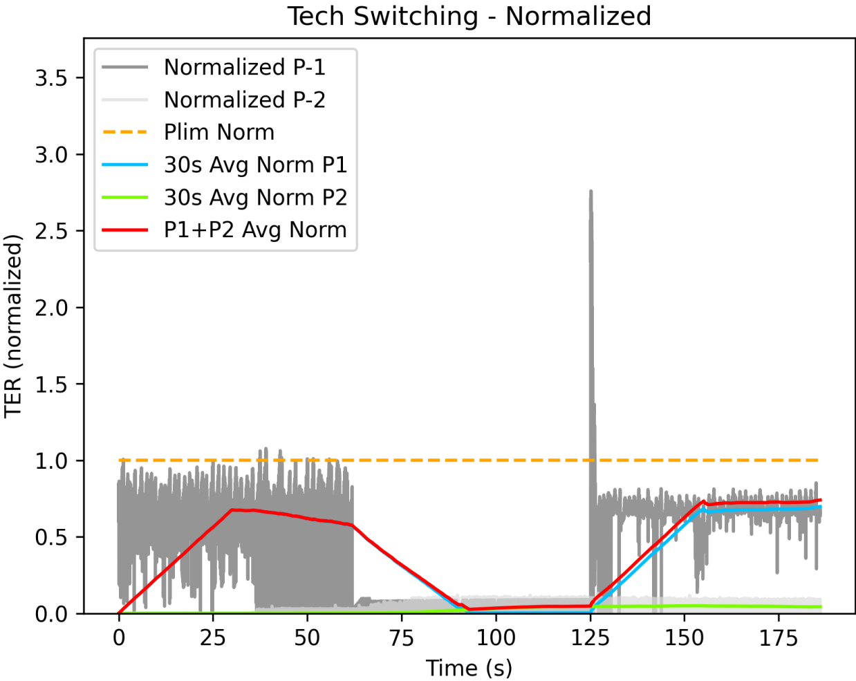
Figure 4-7: Change in Technology and Band Validation
