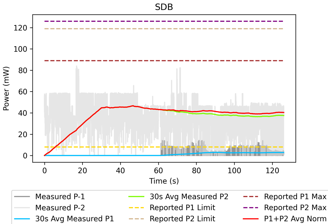
Figure 4-16: Wi-Fi 2.4 GHz to Wi-Fi 2.4 GHz + 6 GHz Plot
