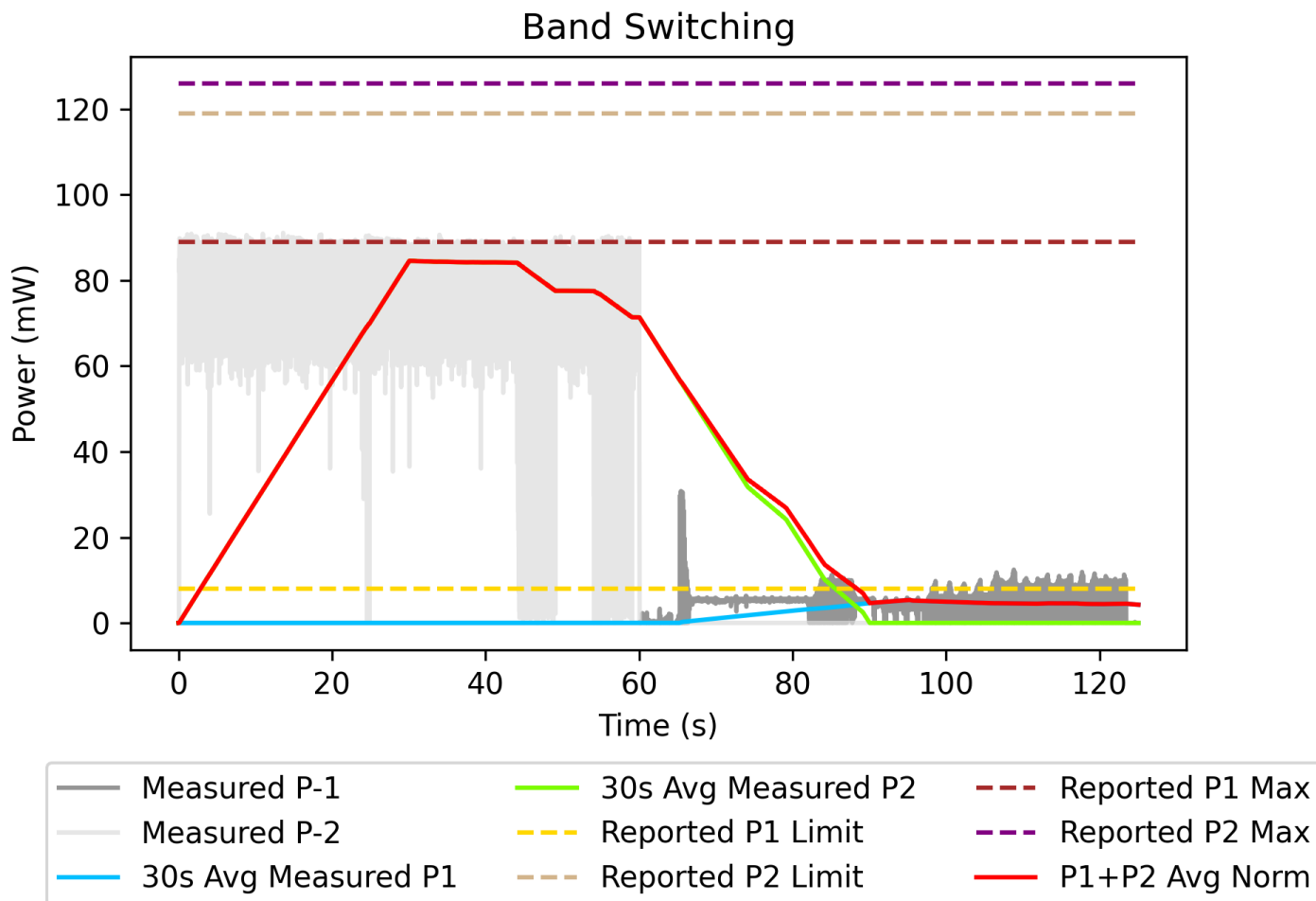
Figure 4-14: Wi-Fi 2.4GHz to 6GHz Plot
