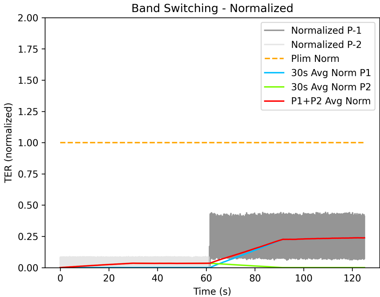
Figure 4-19: Figaro 5G Antenna/Band Switch Validation Plot
