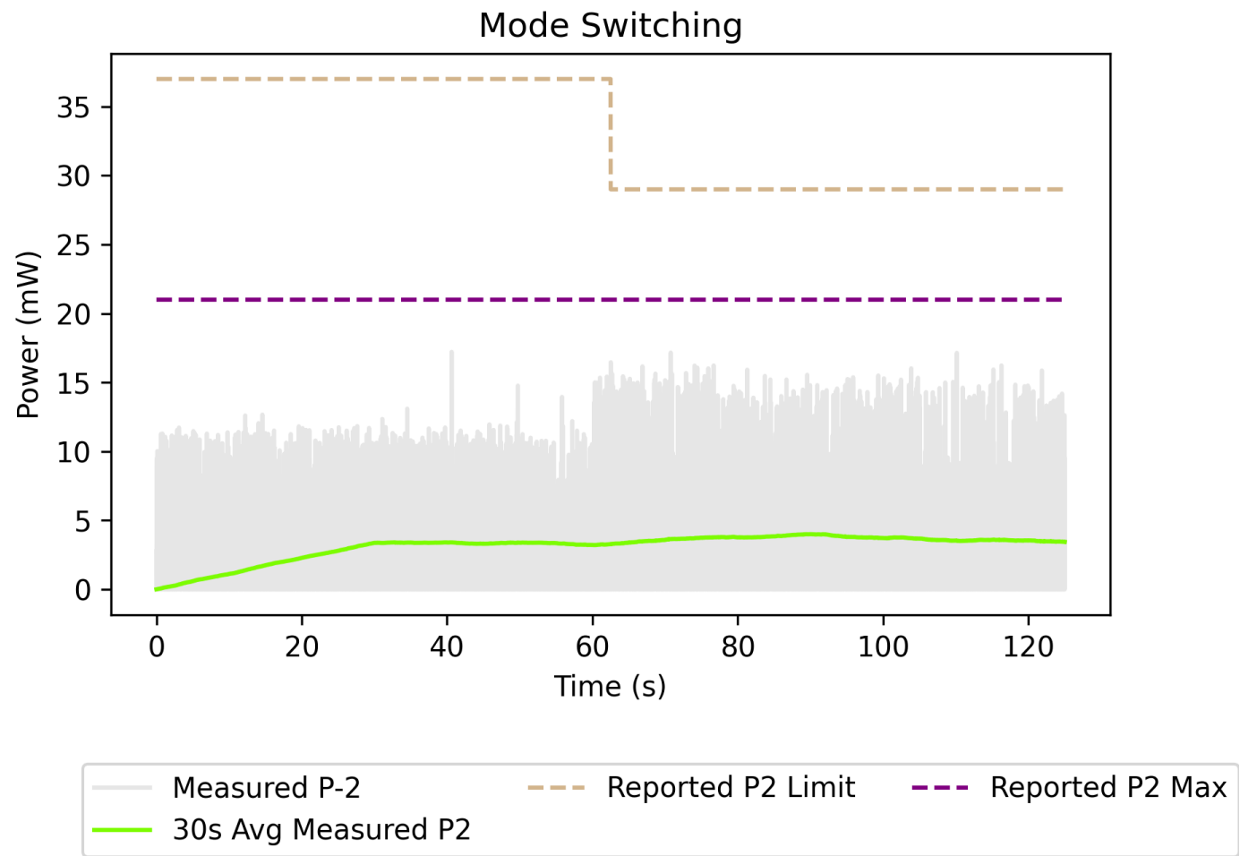
Figure 4-12: BT Power State 5 to Power State 6 Plot
