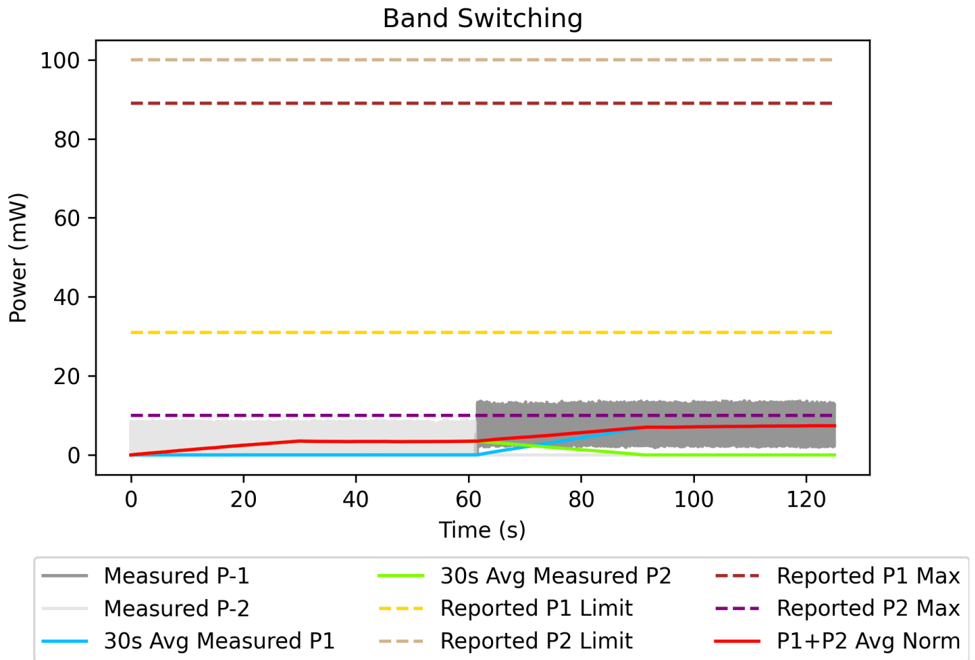
Figure 4-18: Figaro 5G Antenna/Band Switch Plot
