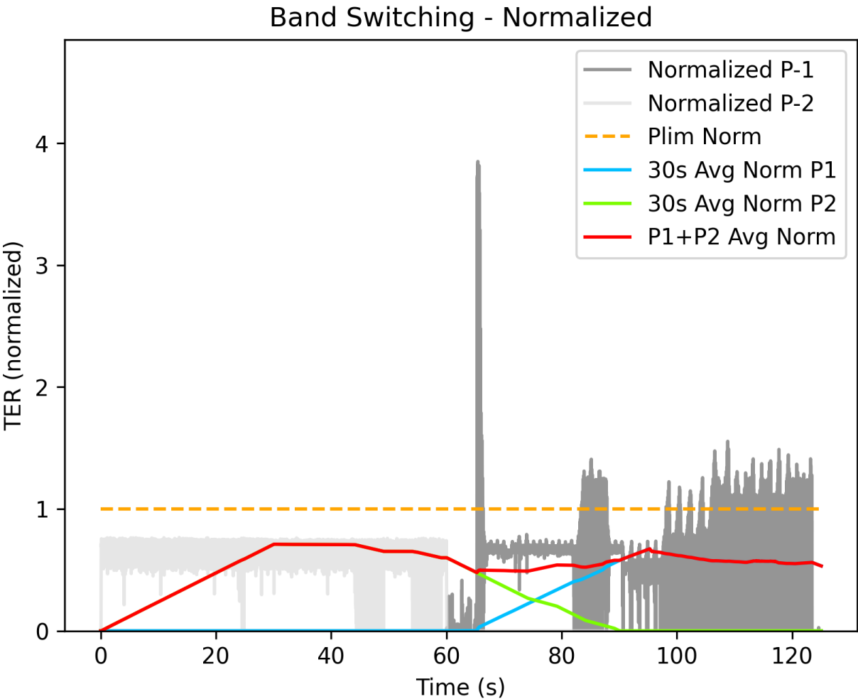
Figure 4-15: Band Switch Validation
