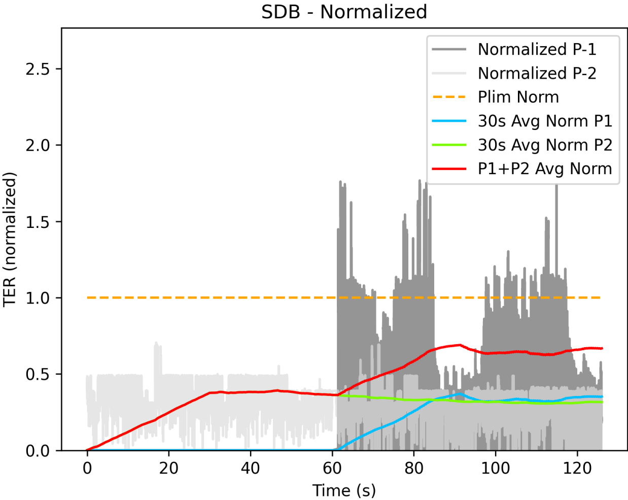
Figure 4-17: Wi-Fi 2.4 GHz to Wi-Fi 2.4 GHz + 6 GHz Validation
