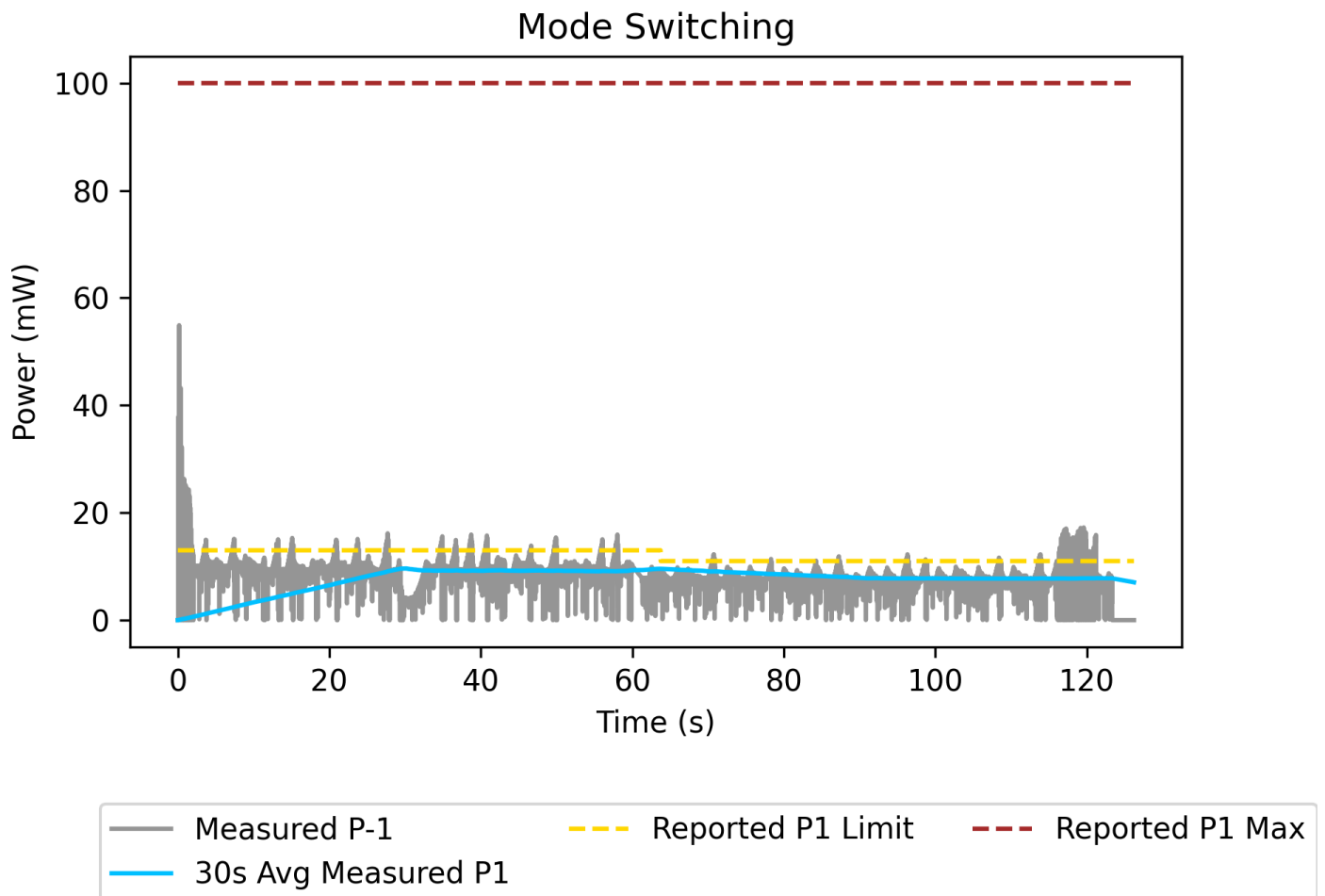
Figure 4-10: Wi-Fi Power State 3 to Power State 4 Plot
