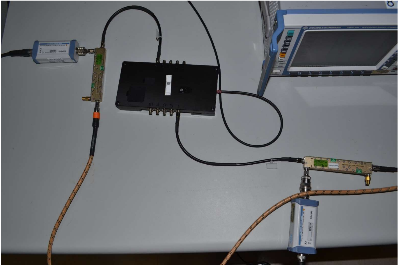
Figure A-2 CMW Conducted power test measurement Setup - Dual port - Uplink Carrier Aggregation case
