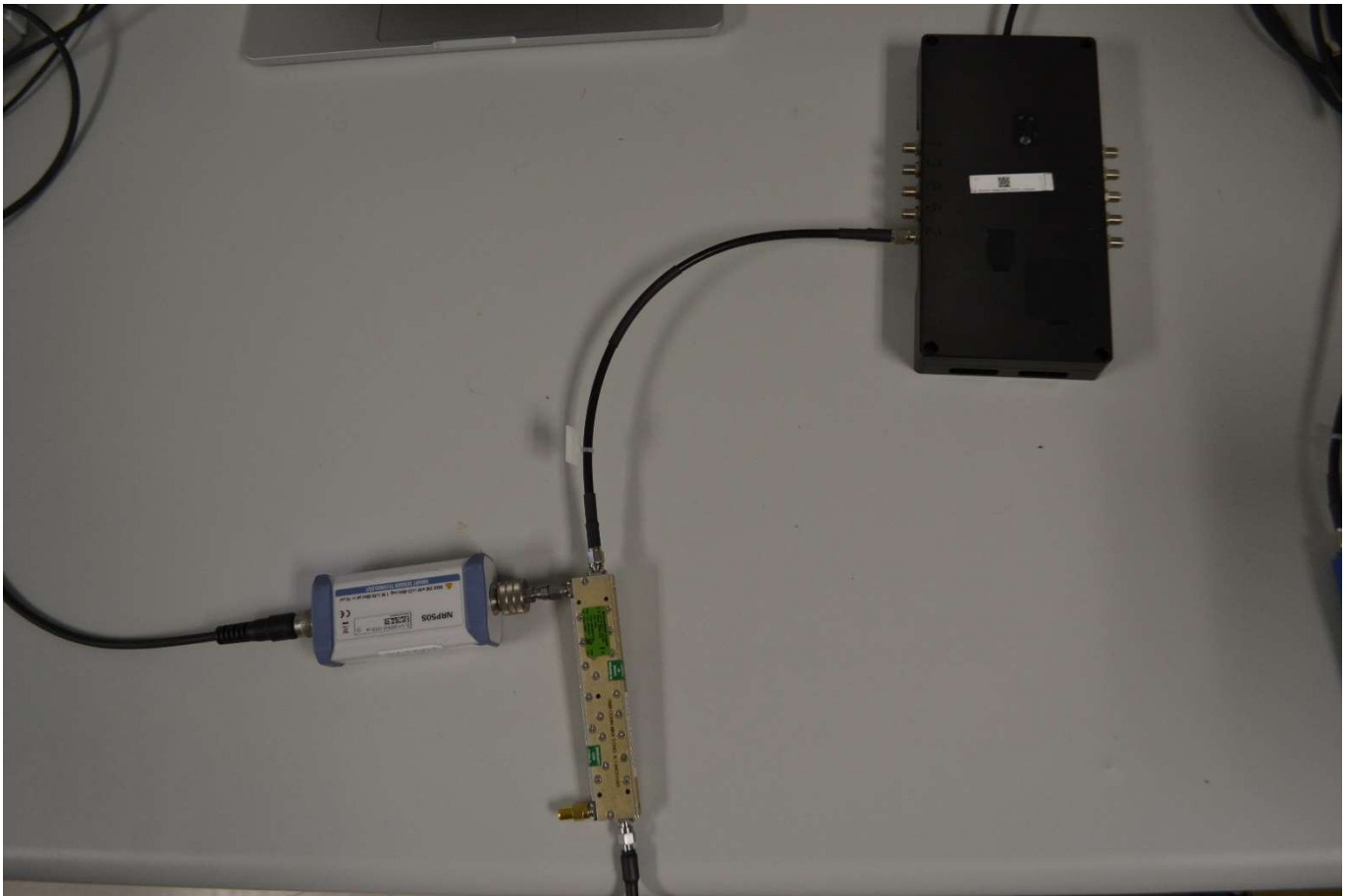
Figure A-3 UXM Conducted power test measurement setup – Single Port
