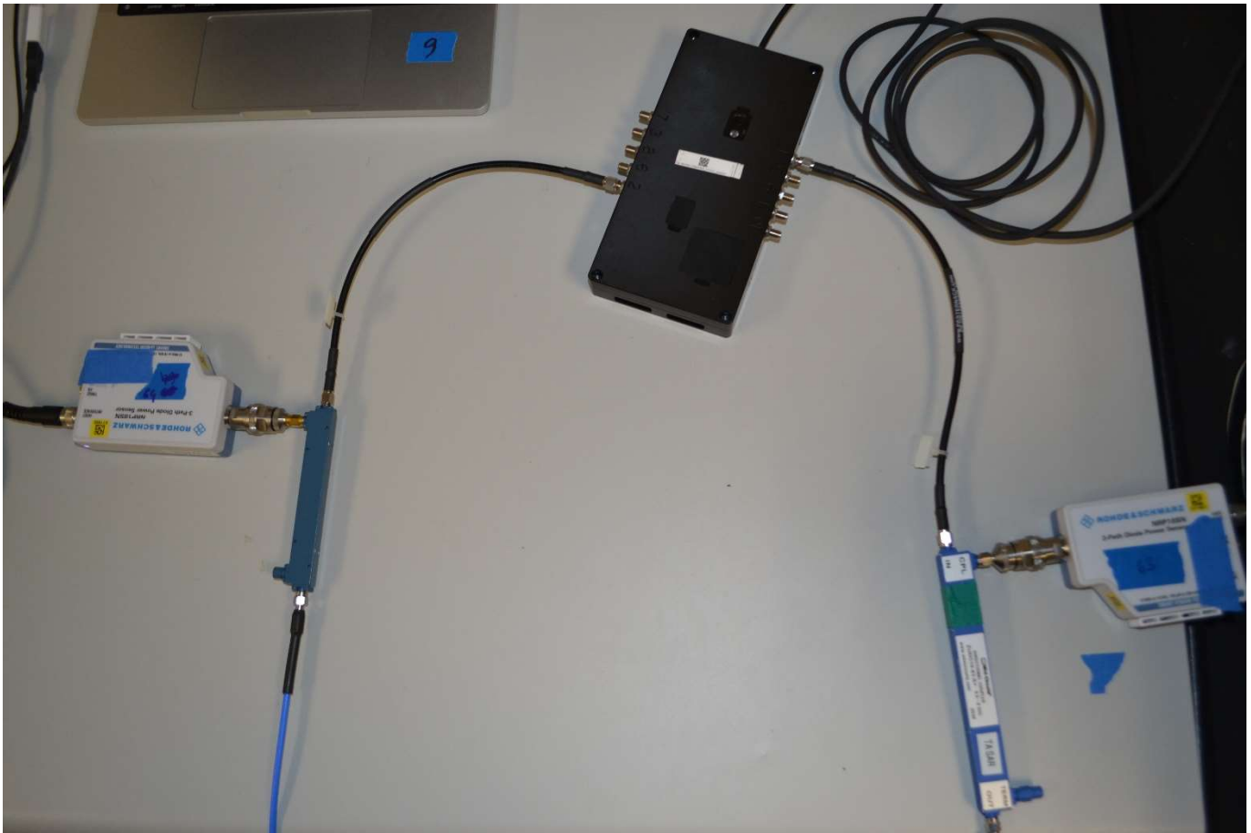
Figure A-4 UXM Conducted power test measurement setup – Dual Port
