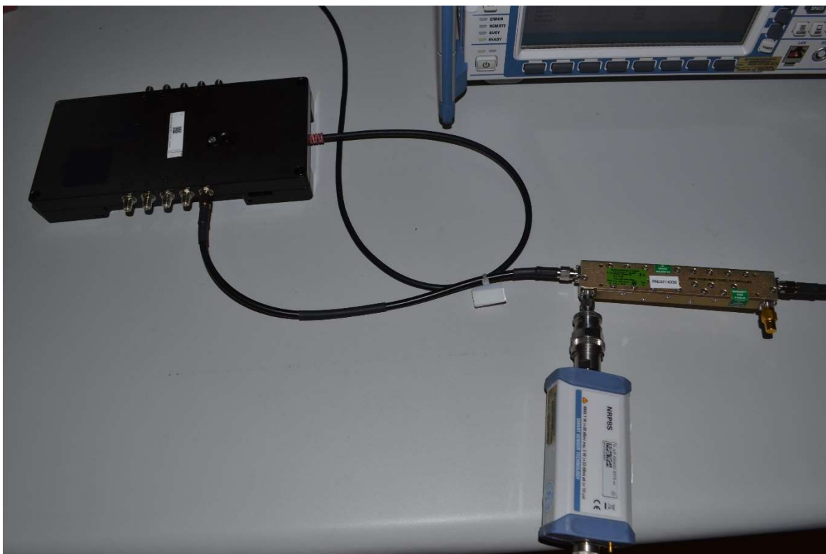
Figure A-1 CMW Conducted power test measurement setup – Single Port
