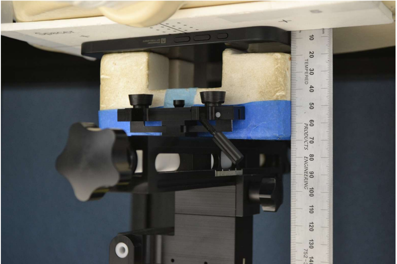
Figure A-5 DASY Radiated power - Linearity Check test measurement setup – Body - Rear
