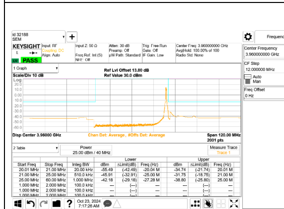
5G NR n77 40MHz BPSK High Channel RB1-05
