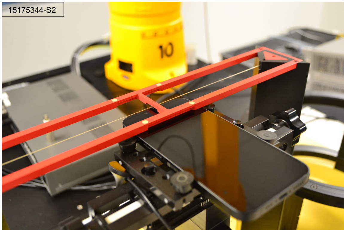
Photograph 1: Front View of the DUT SAR 10
