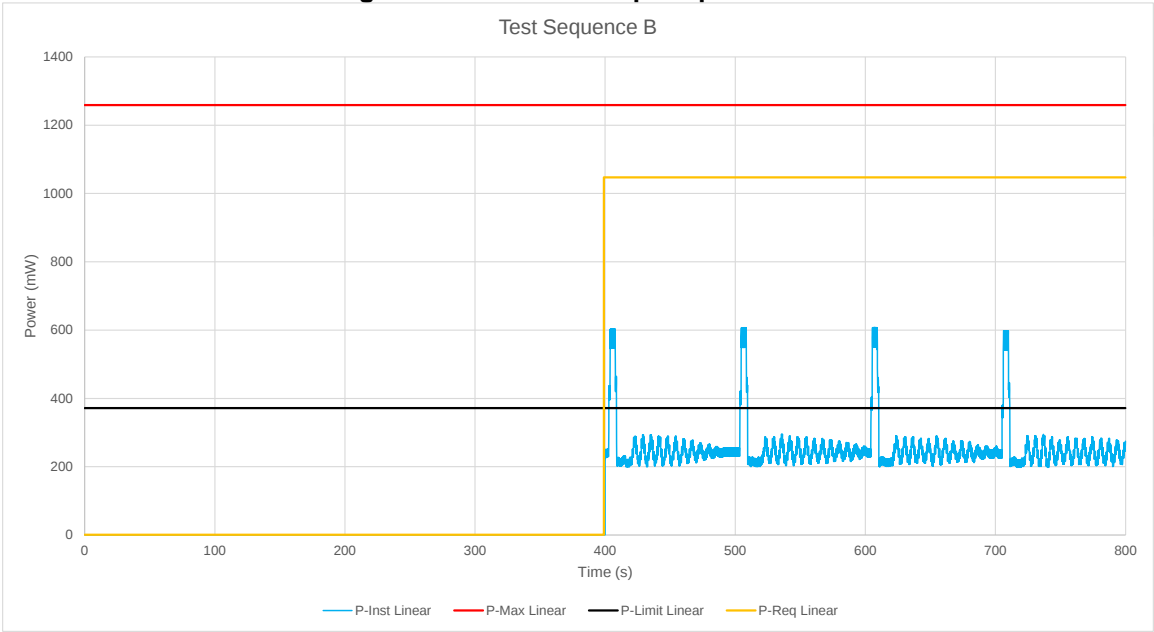
Figure 5-7: GSM P[n] vs. P Limit 1b Validation
