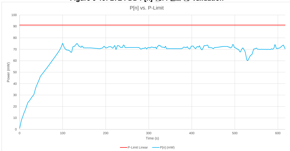
Figure 5-19: LTE FDD P[n] vs. P_{Limit} 1c Validation
