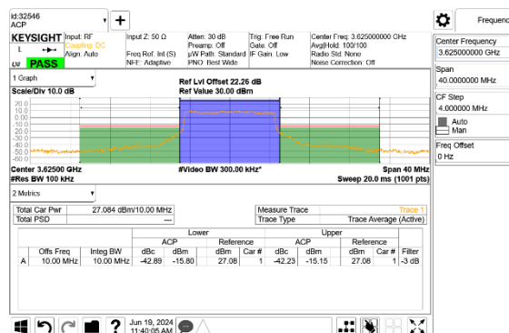
LTE B48 10MHz QPSK Middle Channel RB50-0
