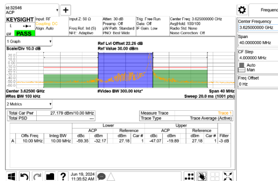
LTE B48 10MHz QPSK Middle Channel RB1-49
