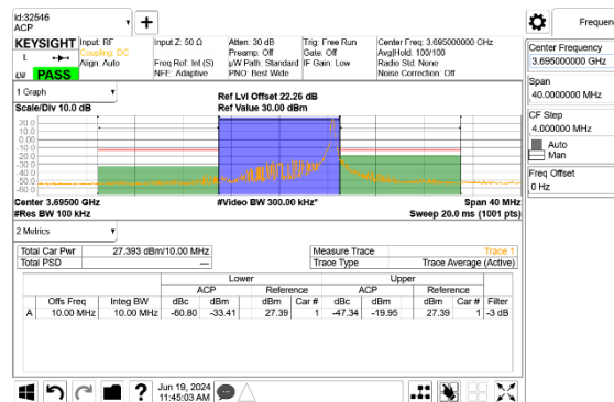
LTE B48 10MHz QPSK High Channel RB1-49
