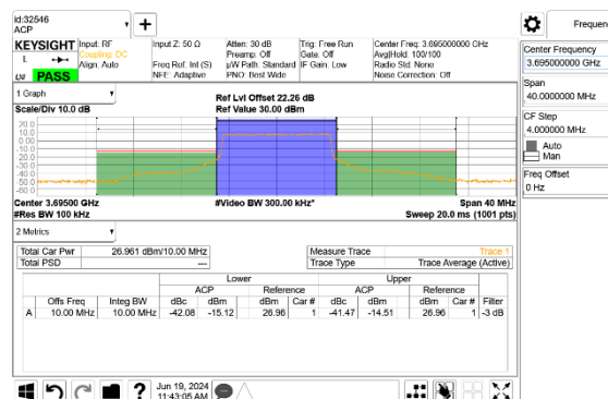
LTE B48 10MHz QPSK High Channel RB50-0
