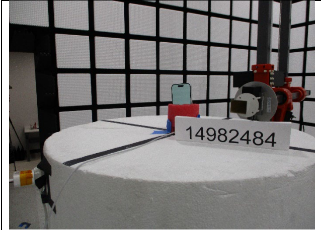
26.5-40 GHz (FRONT)
