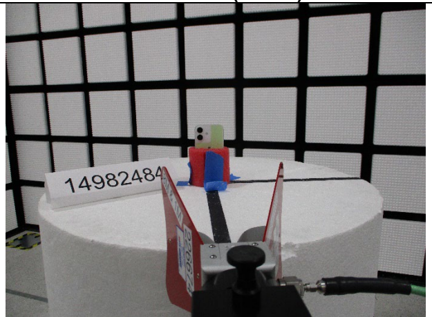
9-18 GHz (Back)
