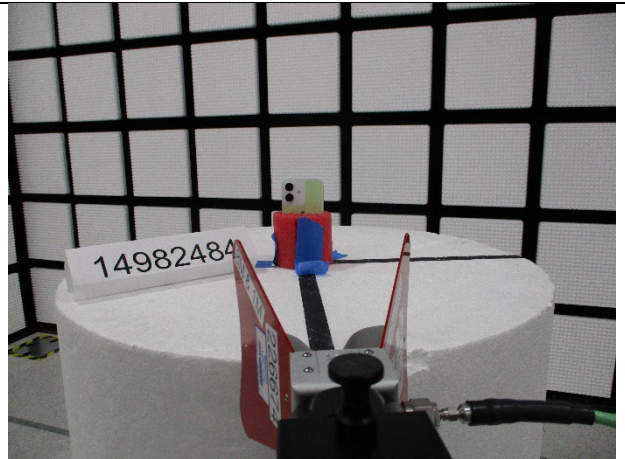
0.96-6GHz (BACK)
