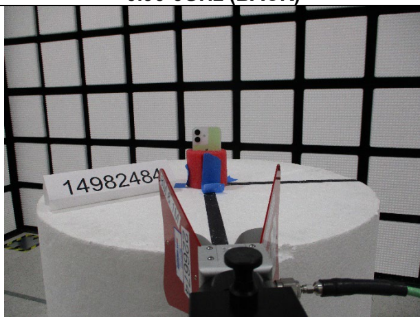
9-18 GHz (Back)
