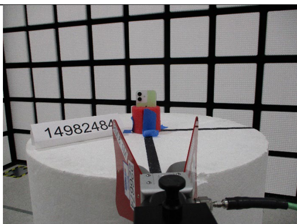
0.96-6GHz (BACK)
