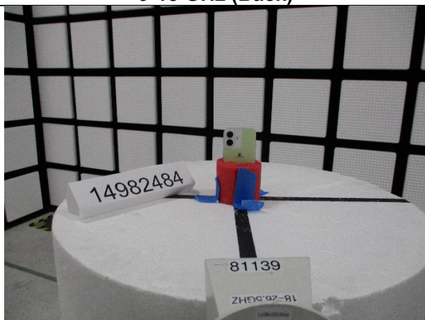
18-26.5 GHz (BACK)
