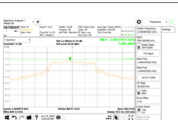
LTE B53 10MHz QPSK Middle Channel RB1-0, ID:32546
