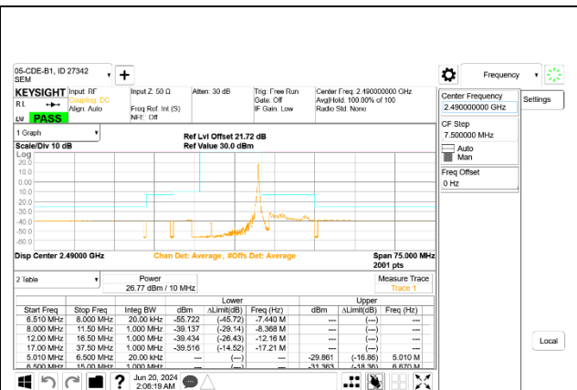
LTE B53 10MHz QPSK High Channel RB1-49
