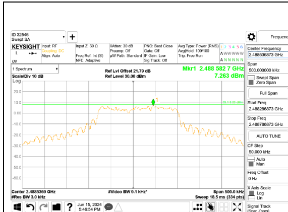
LTE B53 1.4MHz QPSK Middle Channel RB1-0, ID:32546
