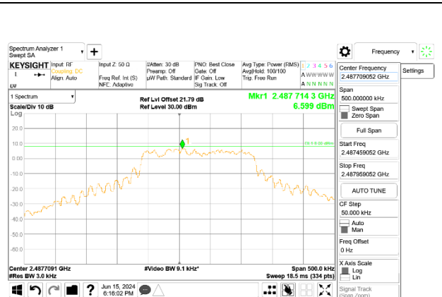
LTE B53 3MHz QPSK Middle Channel RB1-0, ID:32546
