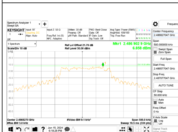
LTE B53 5MHz QPSK Middle Channel RB1-0, ID:32546
