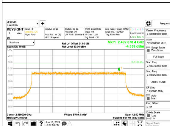
LTE B53 10MHz QPSK Middle Channel RB50-0
