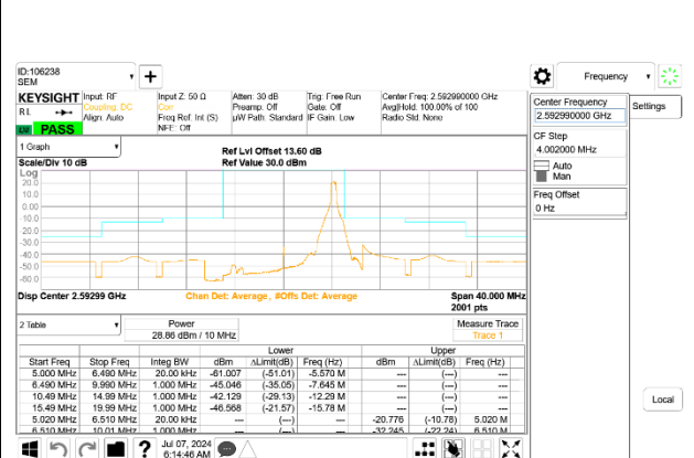
5G NR n41 10MHz BPSK Middle Channel RB1-23
