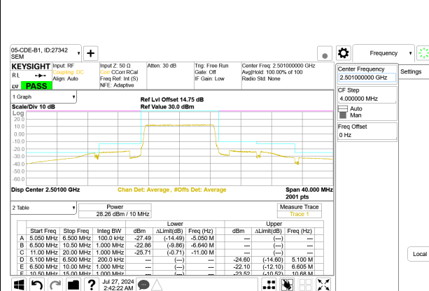
LTE B41 10MHz QPSK Low Channel RB50-0
