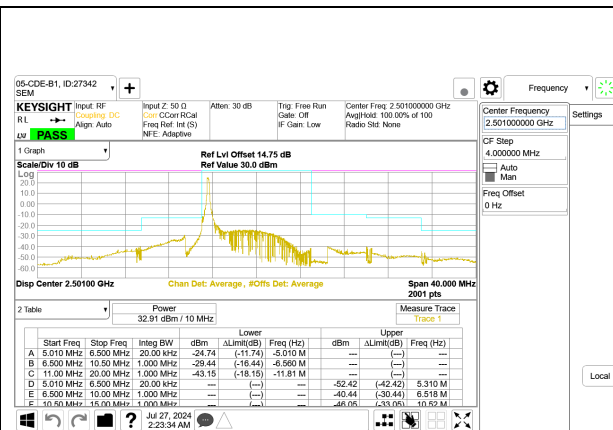
LTE B41 10MHz QPSK Low Channel RB1-0
