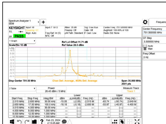
5G NR n12 5MHz BPSK Low Channel RB1-0 ID:28567
