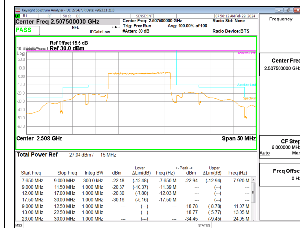
5G NR n7 15MHz BPSK Low Channel RB75-0
