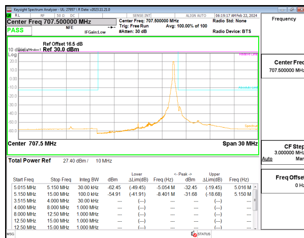
LTE B12 10MHz QPSK Middle Channel RB1-49
