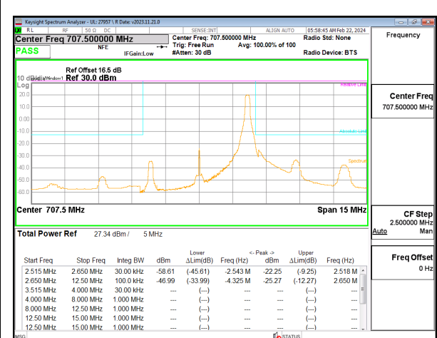
LTE B12 5MHz QPSK Middle Channel RB1-24
