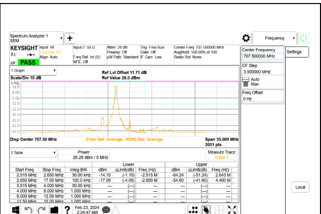
5G NR n12 5MHz BPSK Middle Channel RB1-0 ID:28567
