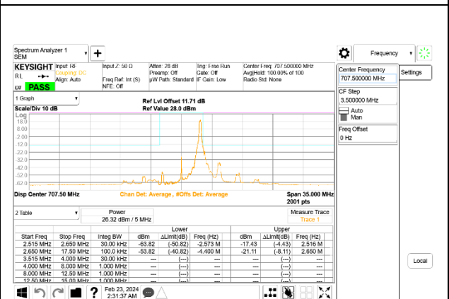
5G NR n12 5MHz BPSK Middle Channel RB1-24 ID:28567
