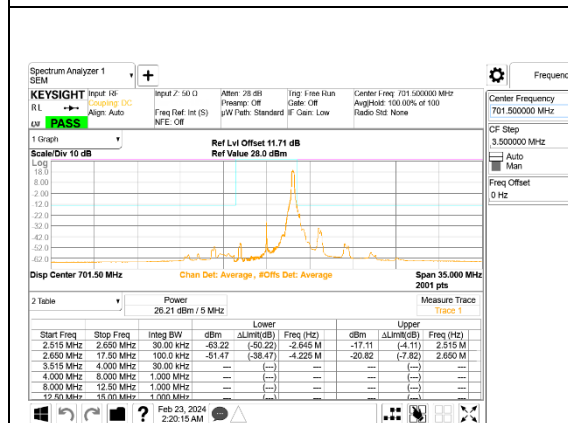
5G NR n12 5MHz BPSK Low Channel RB1-24 ID:28567
