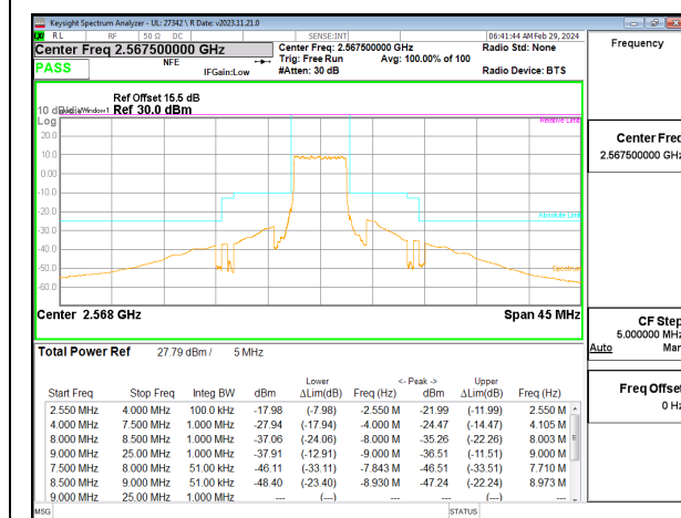
5G NR n7 5MHz BPSK High Channel RB25-0
