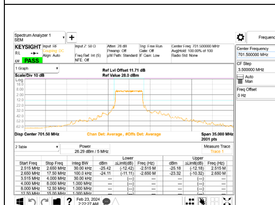
5G NR n12 5MHz BPSK Low Channel RB25-0 ID:28567
