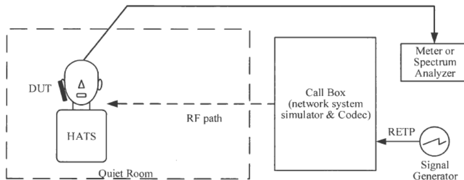
Figure 5-1: Test Arrangement
