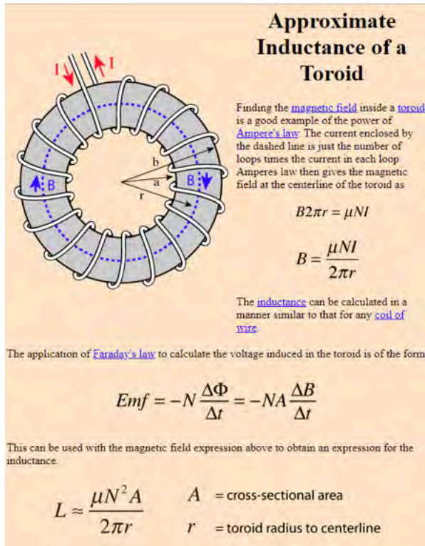
Figure 13: Toroid Model
