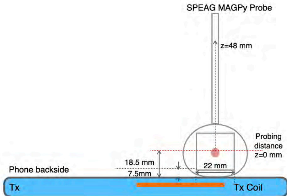
Figure 3: H-field measurement setup for direct exposure case
