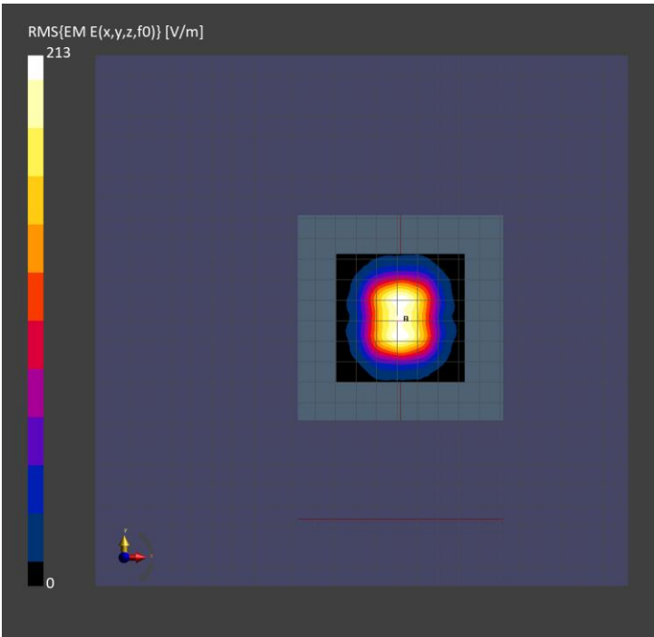
Figure 4-1: 4cm² PD for source validation (worst-case Δ) SAR C
