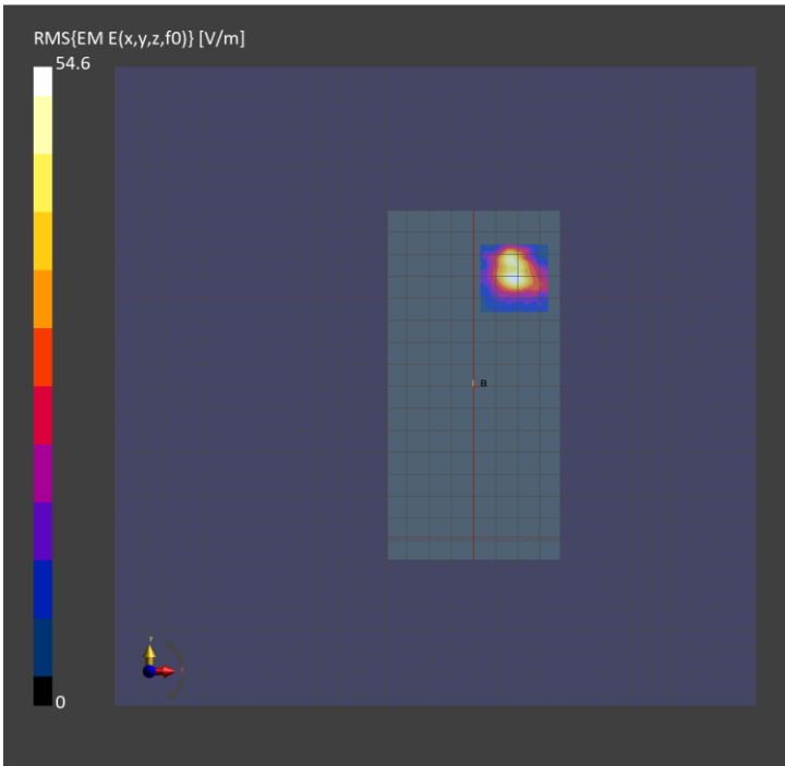
Figure 6-3: Band n261, Beam ID 148, point PD and 4cm² PD, Right
