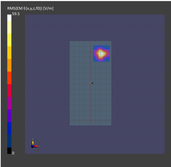
Figure 6-1: Band n258, Beam ID 142, point PD and 4cm² PD, Back
