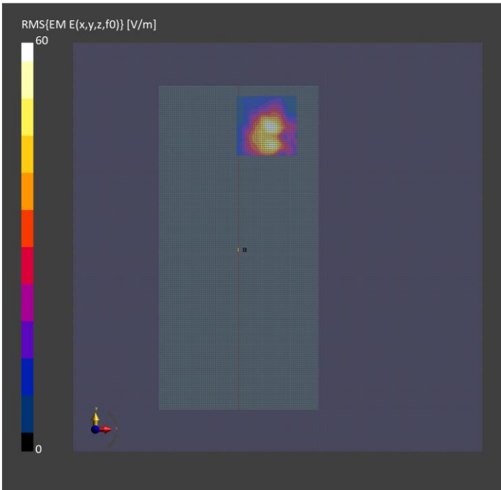
Figure 6-2: Band n260, Beam ID 146, point PD and 4cm² PD, Right
