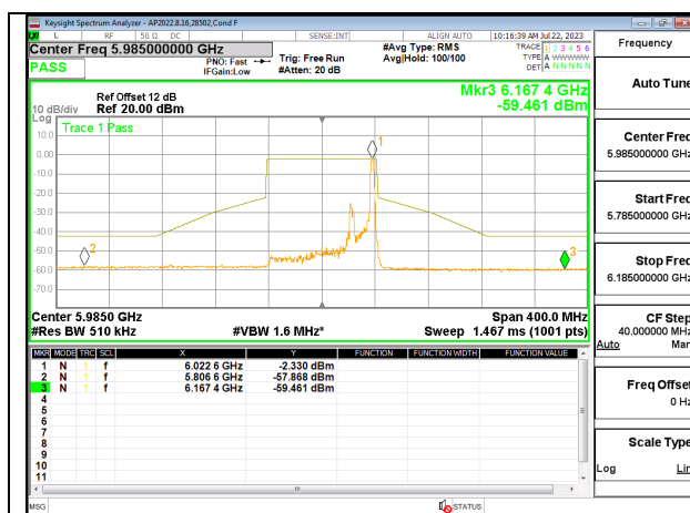
LOW CHANNEL 5985
