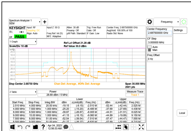
LTE B41 5MHz QPSK High Channel RB1-0, ID:19210
