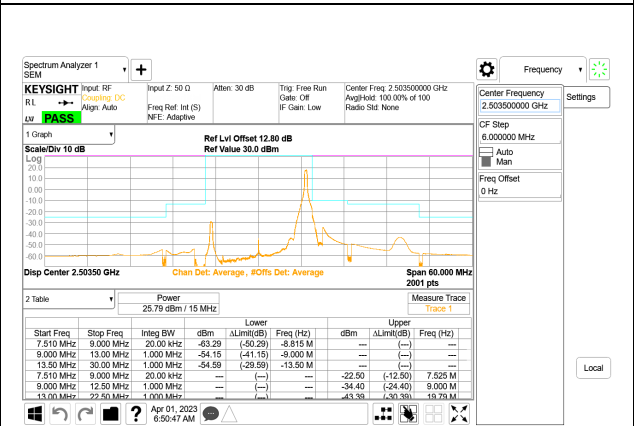
5G NR n41 15MHz BPSK Low Channel RB1-37, ID:19210
