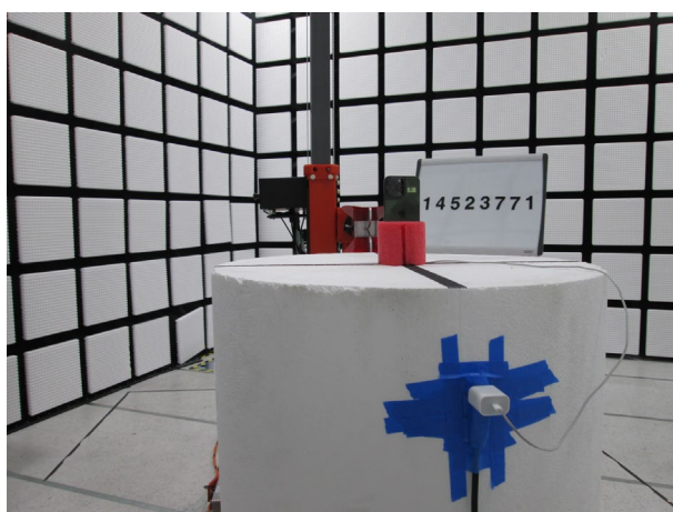
9 – 18 GHz (BACK)
