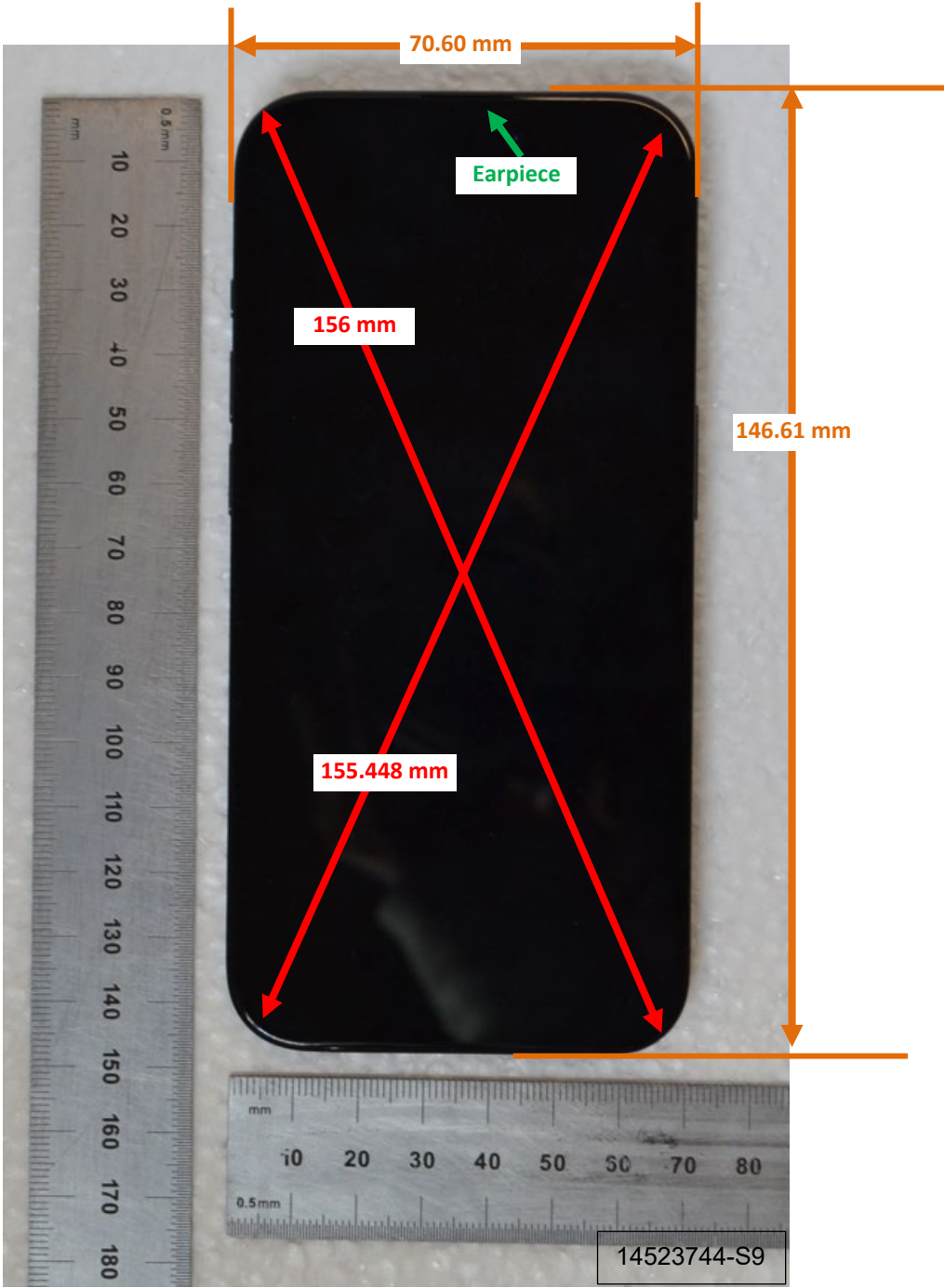
Photograph 1: Overall Dimensions
