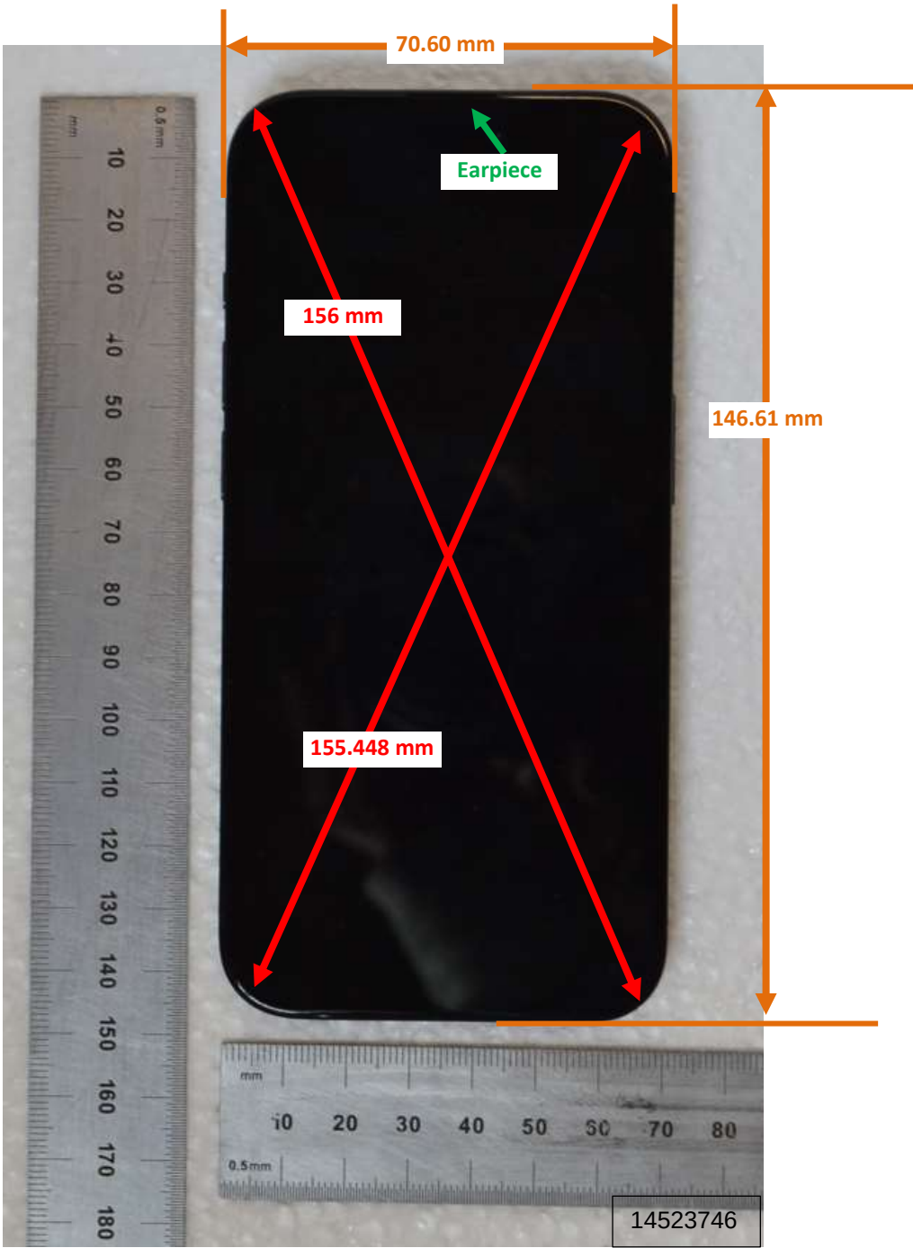
Photograph 1: Overall Dimensions
