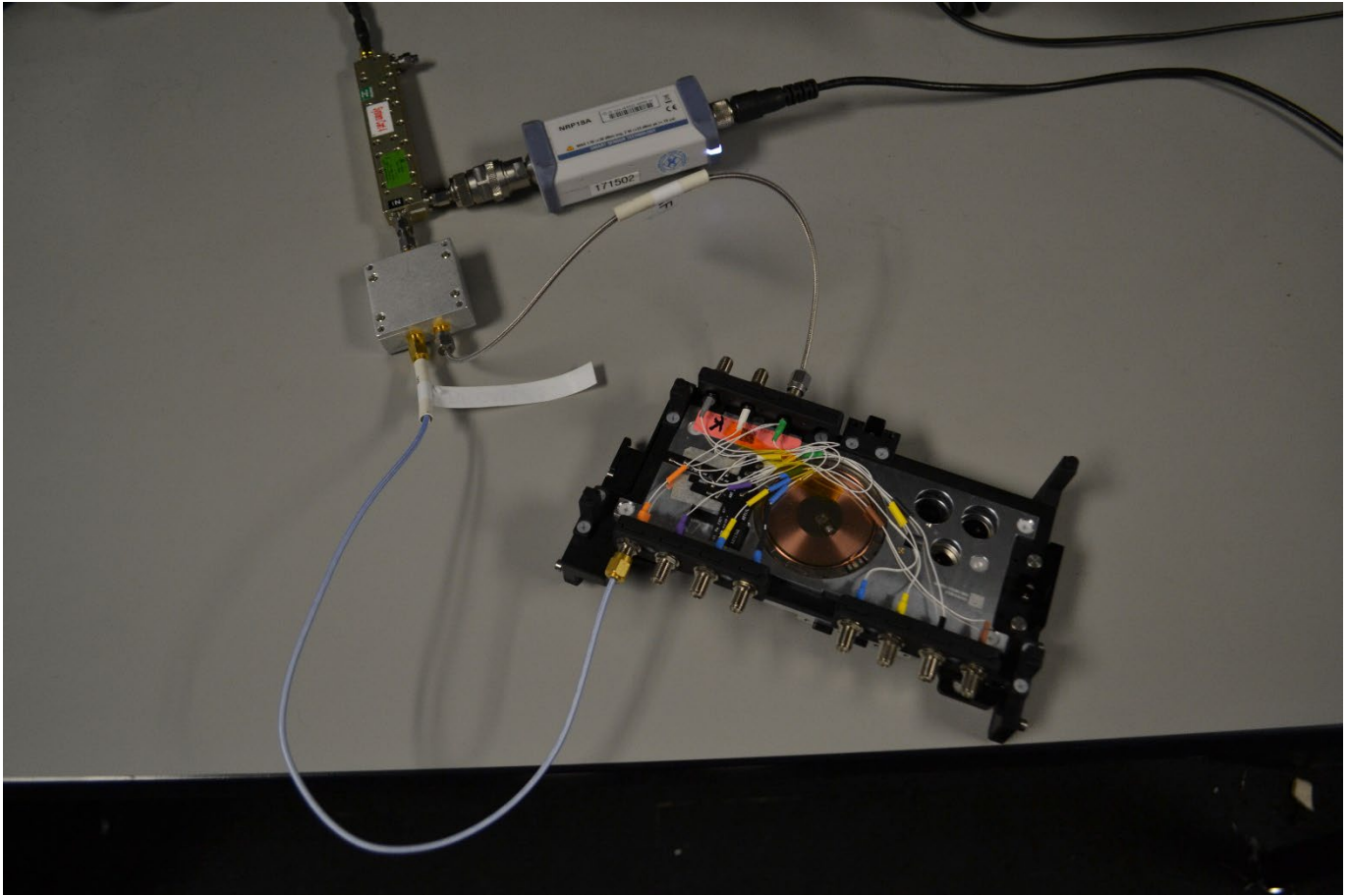
Figure C-2 CMW Conducted power test measurement setup dual port to single Port to call processor, Antenna Switch case
