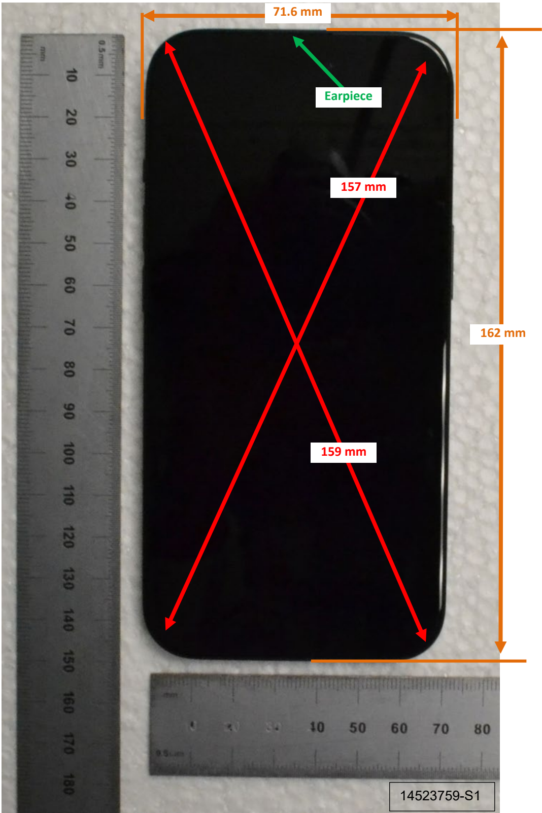
Photograph 1: Overall Dimensions
