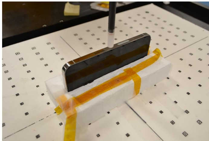
Figure 9-1: Worst-surface of EUT positioned facing up for the mmW beam being tested
