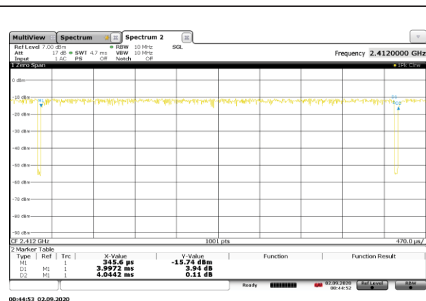
DUTY CYCLE 802.HE20 26T (MCS9)
