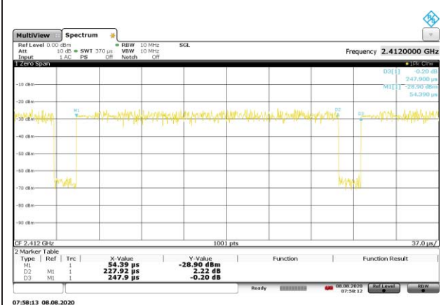
DUTY CYCLE 802.HT20 (MCS7)
