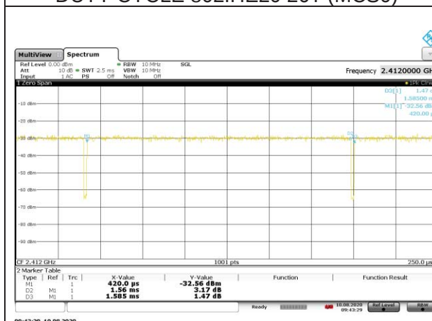
DUTY CYCLE 802.HE20 242T (MCS0)
