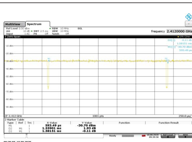
DUTY CYCLE 802.HE20 242T (MCS9)
