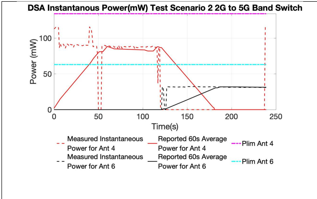
Figure 9 60 Second Average Power vs Time during Band Switch and Instantaneous Power
