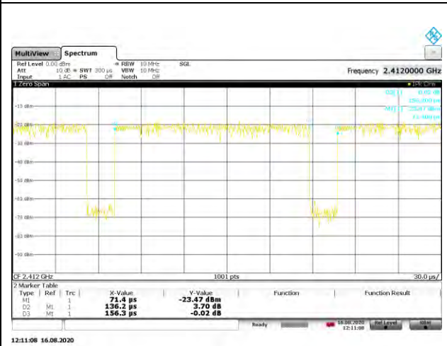
DUTY CYCLE 802.11n HT20 2Tx MCS7
