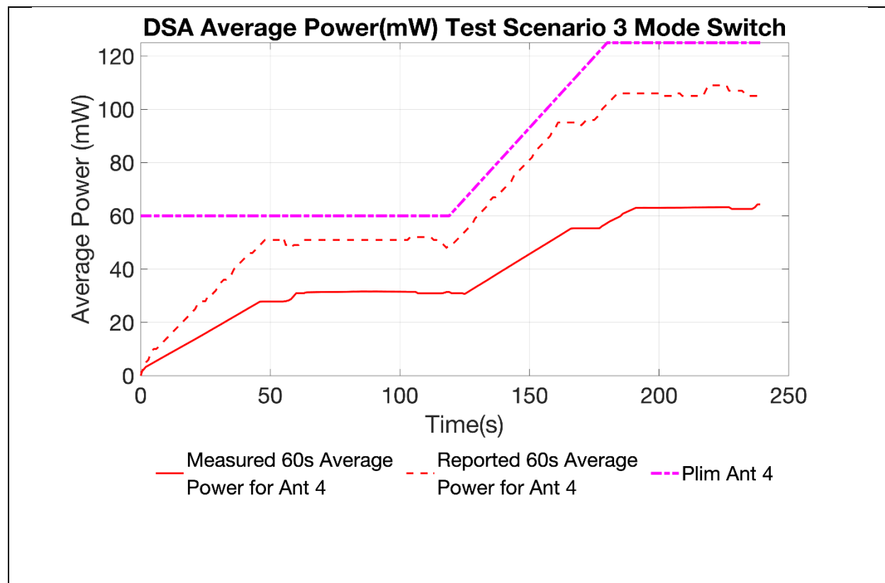
Figure 11 60 Second Average Power vs Time during Mode Switch
