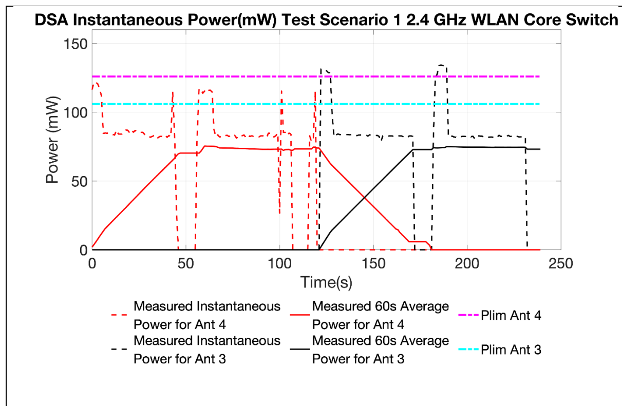
Figure 3 60 Second Average Power vs Time and Instantaneous Power, 2.4GHz
