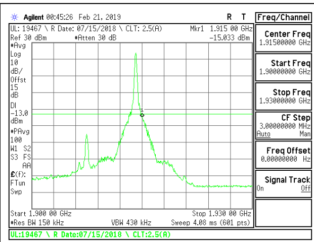
LTE B25 15MHz 16QAM High Channel RB1-74
