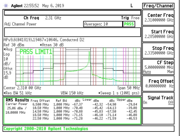
LTE B30 10MHz 16QAM Middle Channel RB1-49
