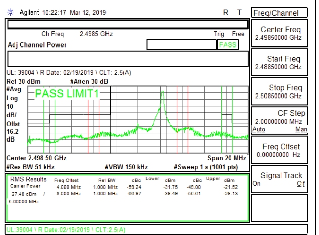
LTE B41 5MHz 16QAM Low Channel RB1-24
