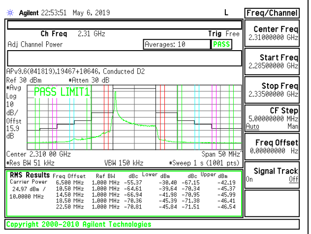
LTE B30 10MHz 16QAM Middle Channel RB1-0
