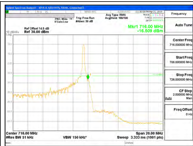
LTE B17 10MHz 16QAM High Channel RB1-49
