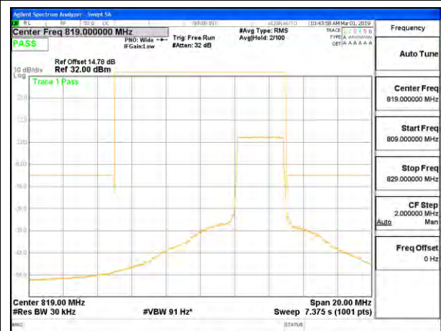
LTE B26 3MHz 16QAM High Channel RB15-0 ID:12491
