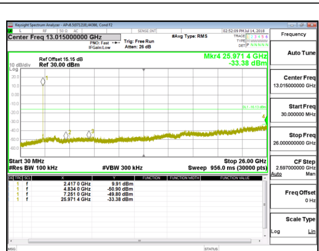
OUT-OF-BAND LOW CHANNEL 2
