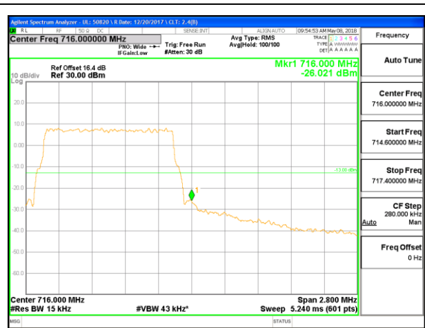
LTE B12 1.4MHz 16QAM High Channel RB6-0
