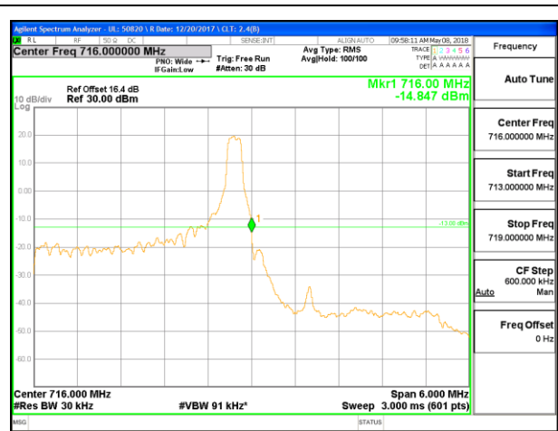
LTE B12 3MHz 16QAM High Channel RB1-14
