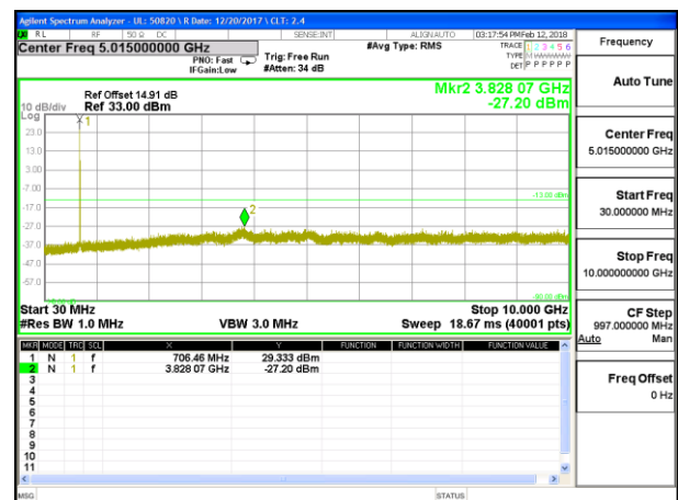
LTE B17 10MHz 16QAM High Channel RB1-0
