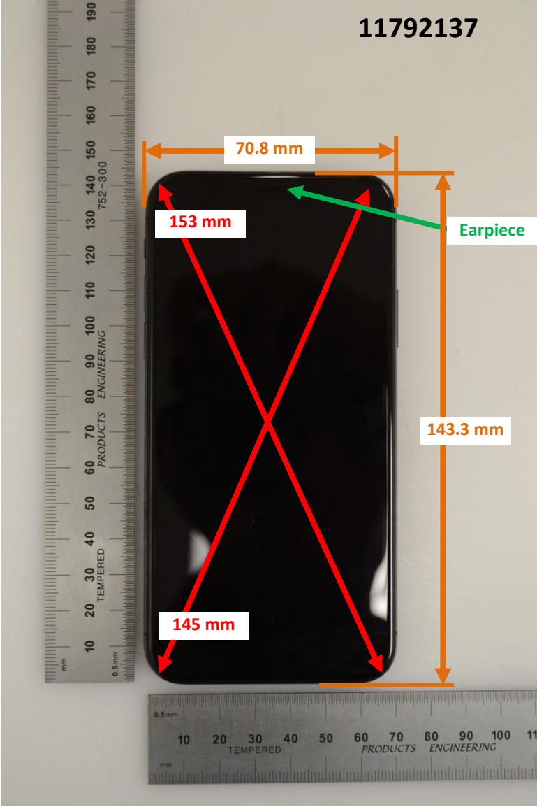
Front View of the DUT
