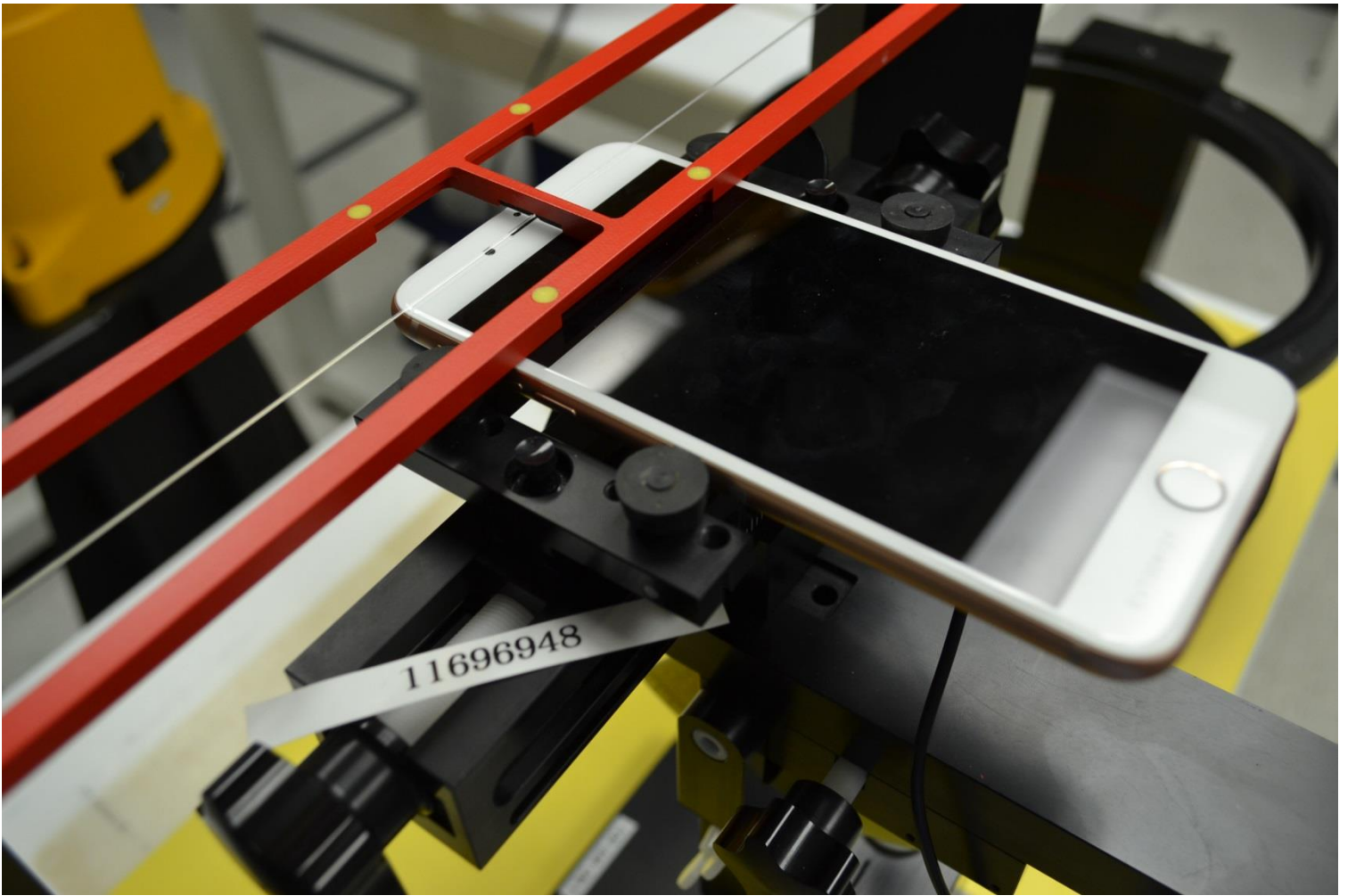
SETUP PHOTO Front View of the DUT
