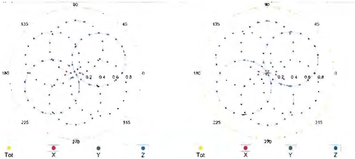
f=600 MHz,TEM
