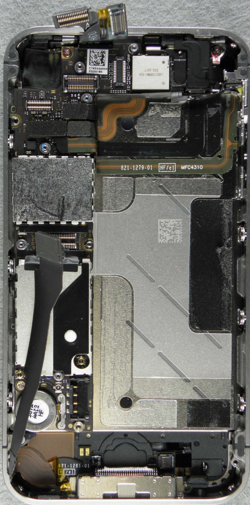
PHOTO 6 FCC ID: BCG-E2422A I/O CONNECTORS REMOVED FROM MAIN BOARD
