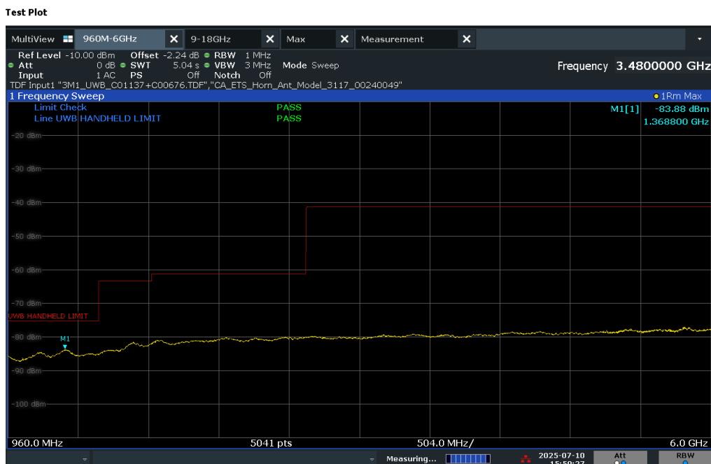
Plot 7-16. FCC Radiated Spurious Emissions 960-6000MHz (Ch. 5, Config 9, Payload 65B Ant. Pol. V)
