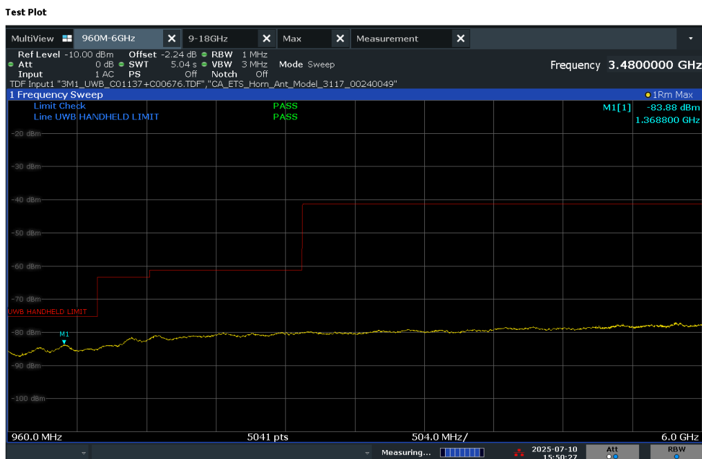
Plot 7-15. FCC Radiated Spurious Emission 960-6000MHz (Ch. 5, Config 9, Payload 65B Ant. Pol. H)
