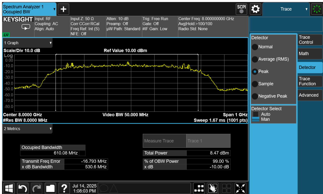
Plot 7-4. ISED 10dBc Bandwidth & 99% Occupied Bandwidth (Ch. 9, Config 9/Payload 65)
