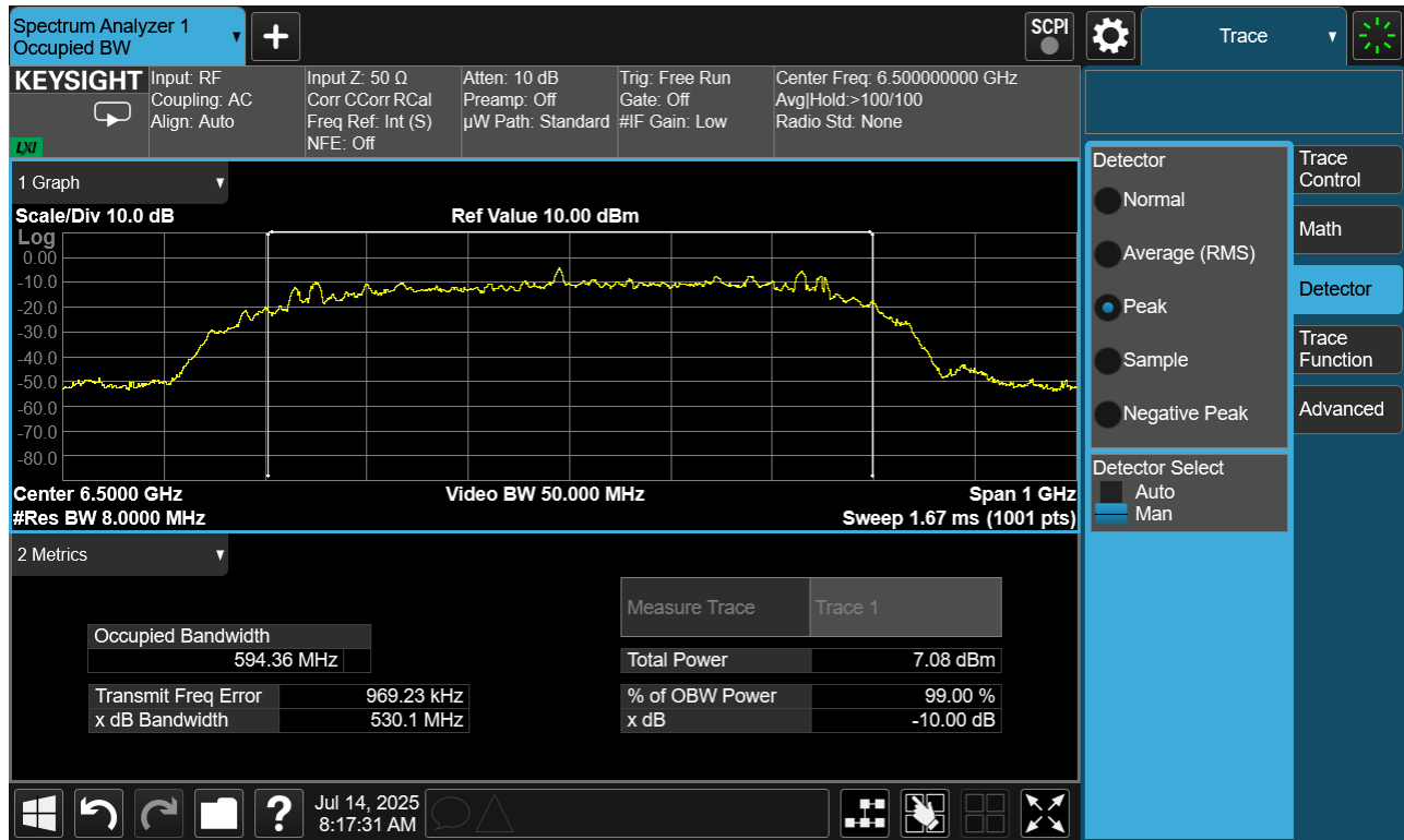
Plot 7-3. ISED 10dBc Bandwidth & 99% Occupied Bandwidth (Ch. 5, Config 9/Payload 65)
