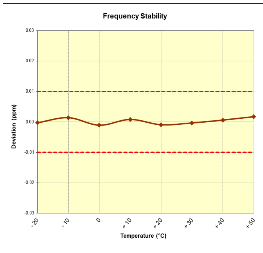
Figure 7-3. Frequency Stability Plot (CE F 212kbps)
