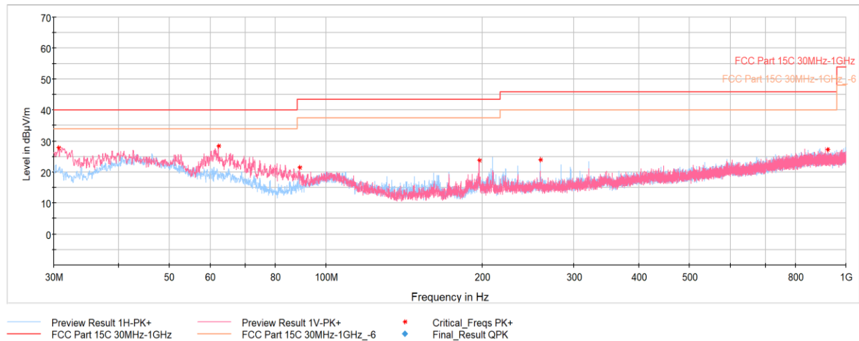
Plot 7-10. Radiated Spurious Emissions 30MHz – 1GHz (CE F 212kbps, with AC/DC Adapter and Magnetic Charger)
