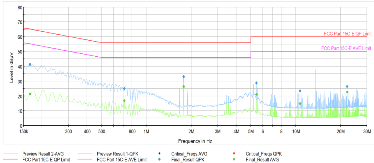
Plot 7-13. AC Line-Conducted Plot (N, CE F 212kbps, with AC/DC Adapter and Magnetic Charger)
