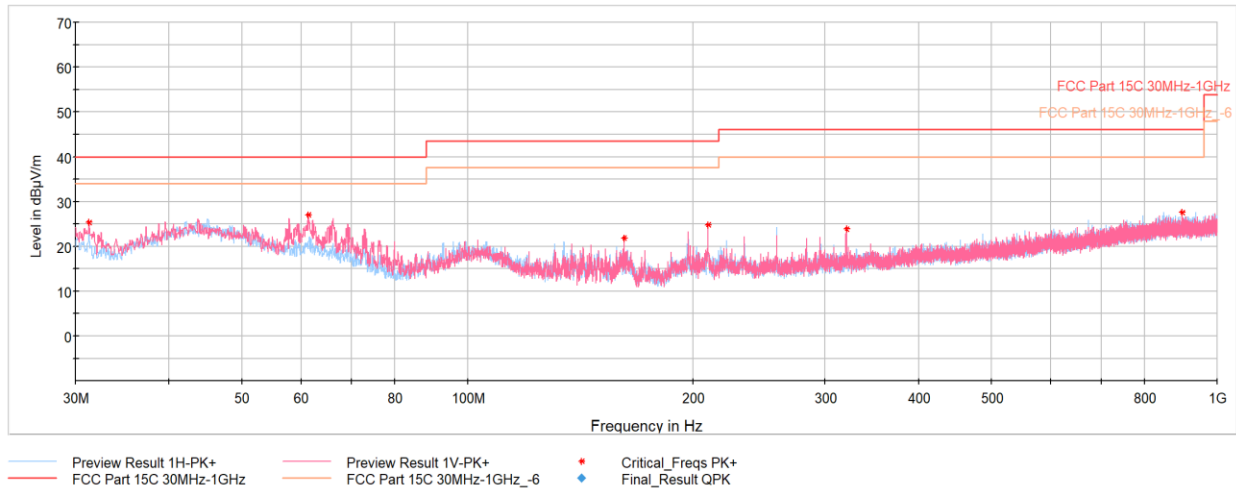
Plot 7-11. Radiated Spurious Emissions 30MHz – 1GHz (Reader A 848kbps, with AC/DC Adapter and Magnetic Charger)
