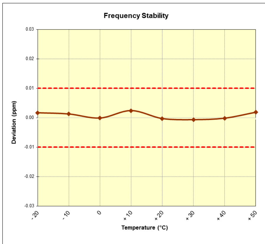
Figure 7-4. Frequency Stability Plot (Reader A 848kbps)
